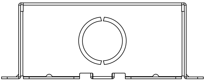
⑥ BOTTOM VIEW
