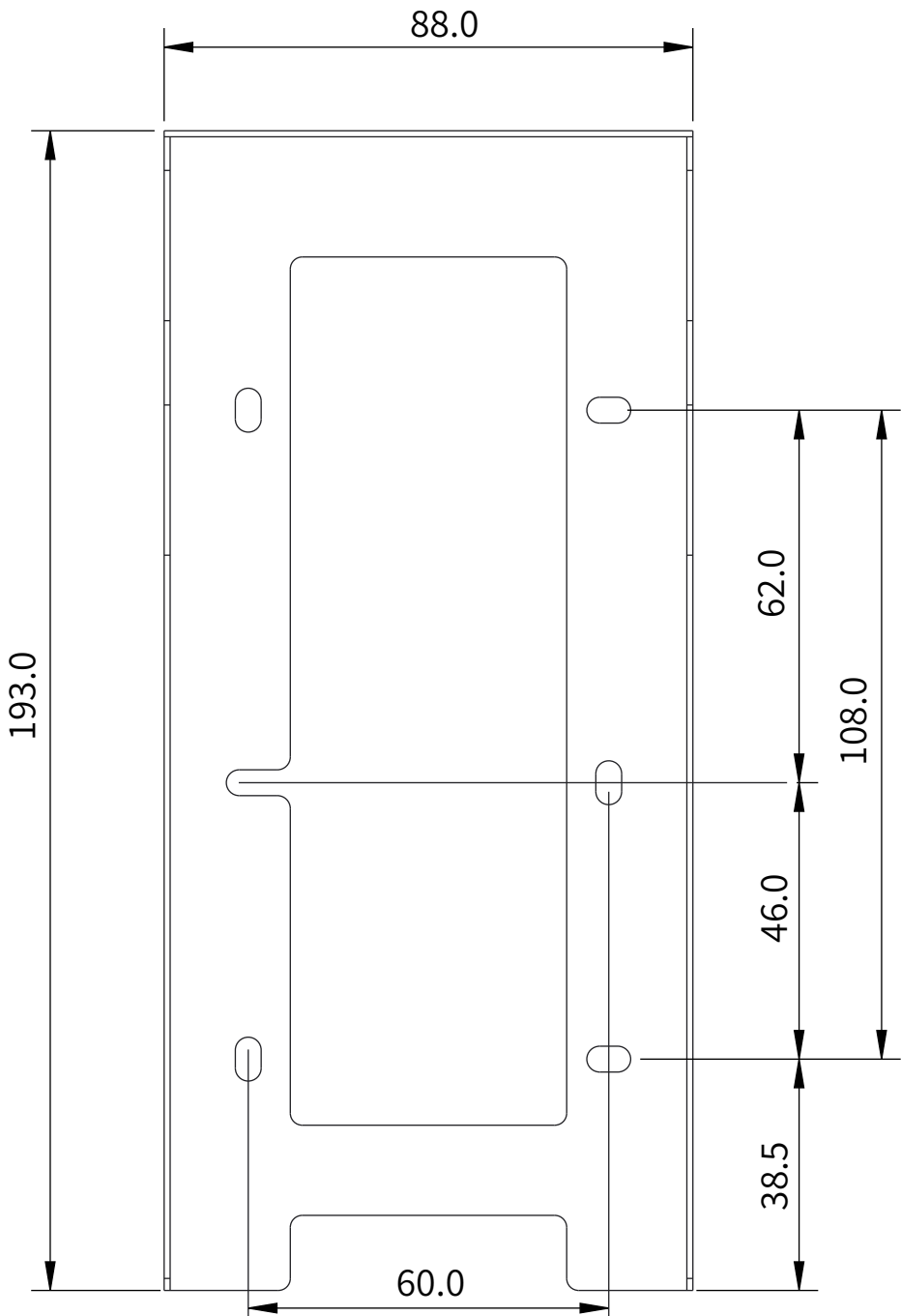
1 FRONT VIEW
