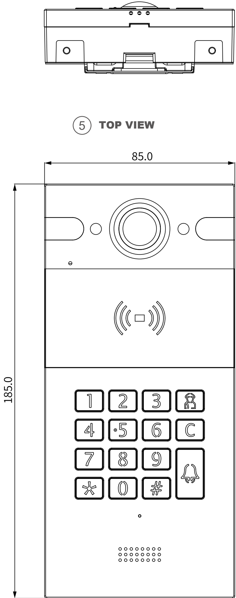
① FRONT VIEW
