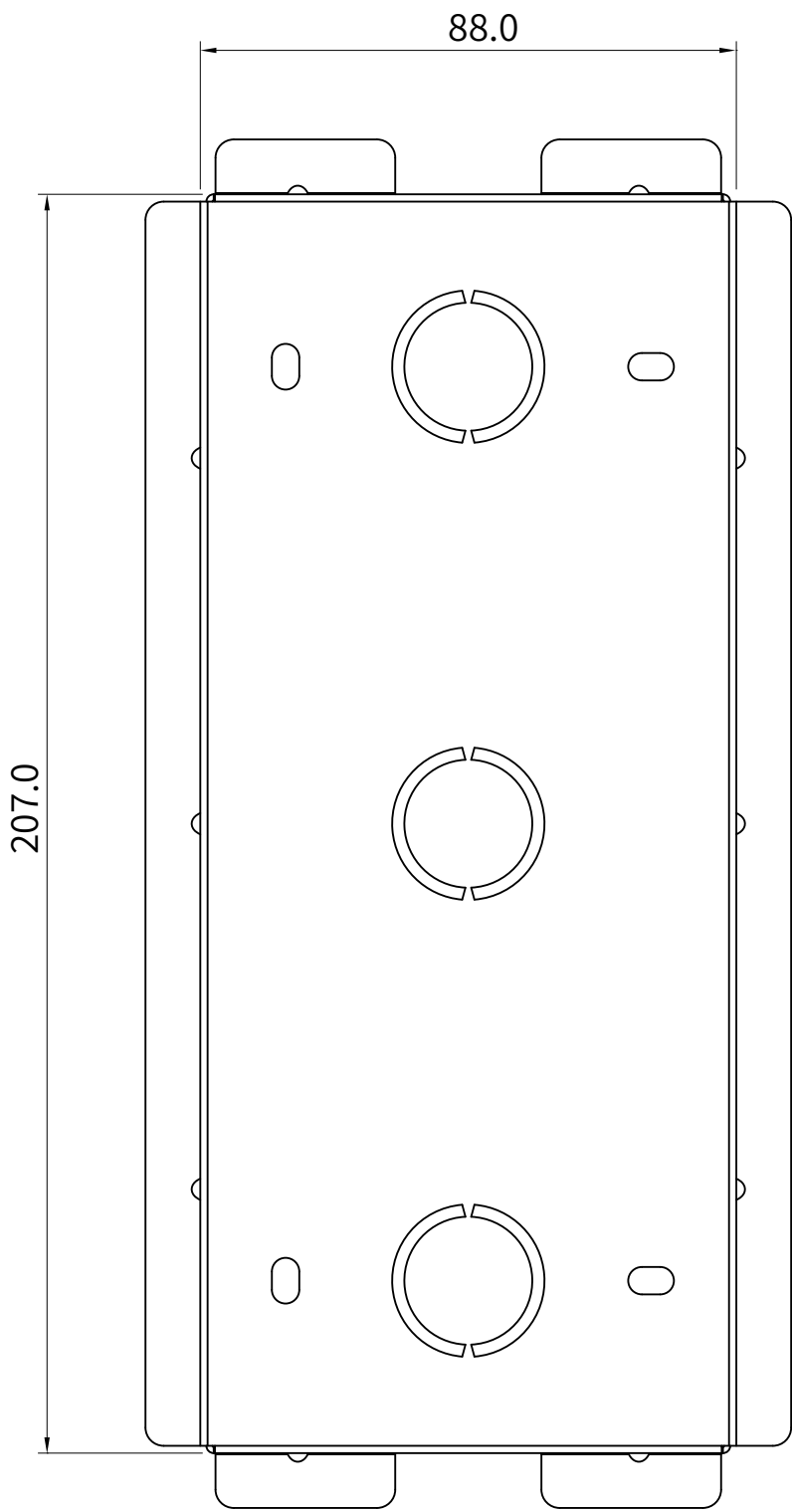
④ BACK VIEW
