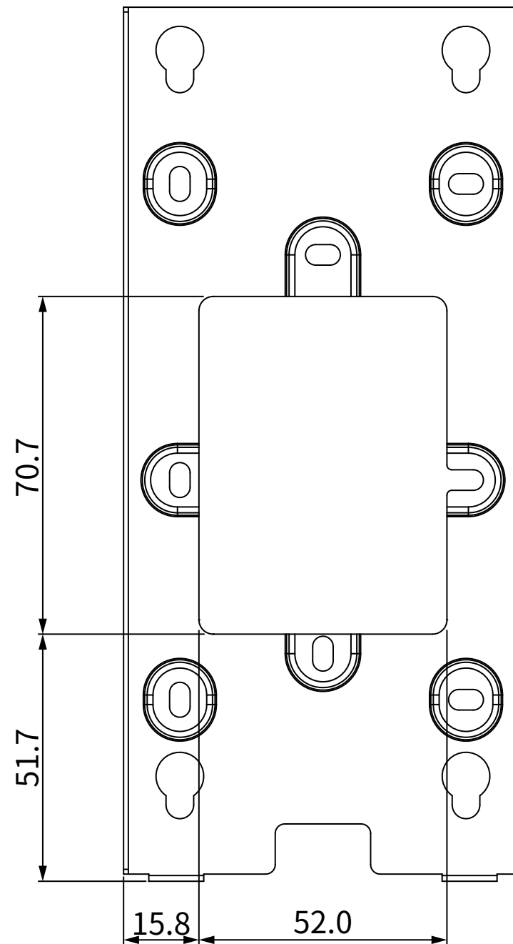
4 BACK VIEW
