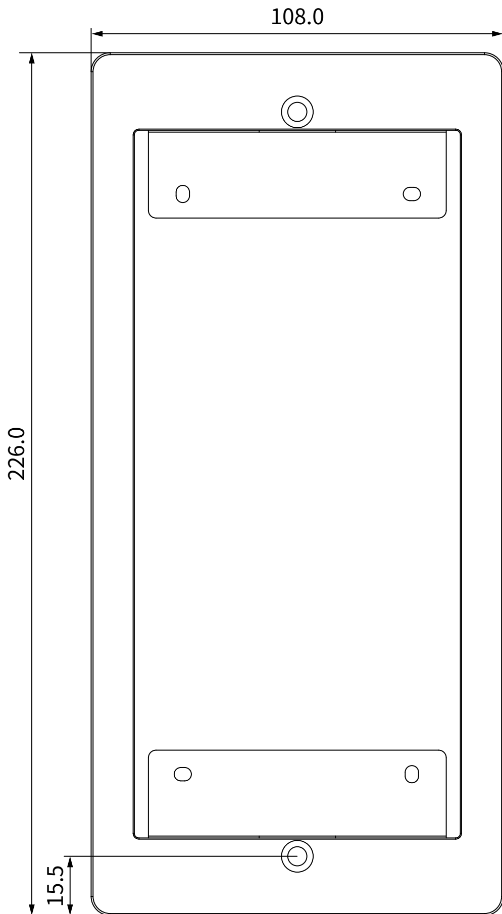
1 FRONT VIEW
