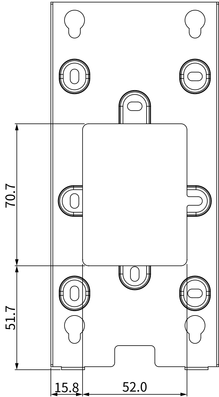
4 BACK VIEW
