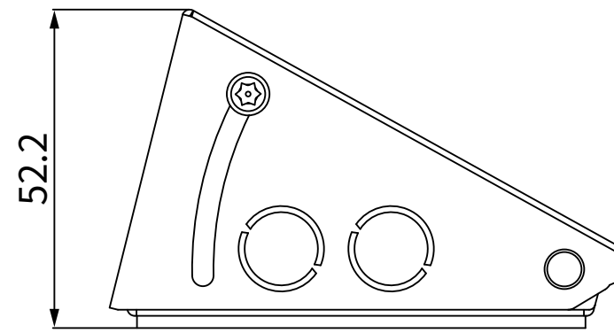
5 TOP VIEW
