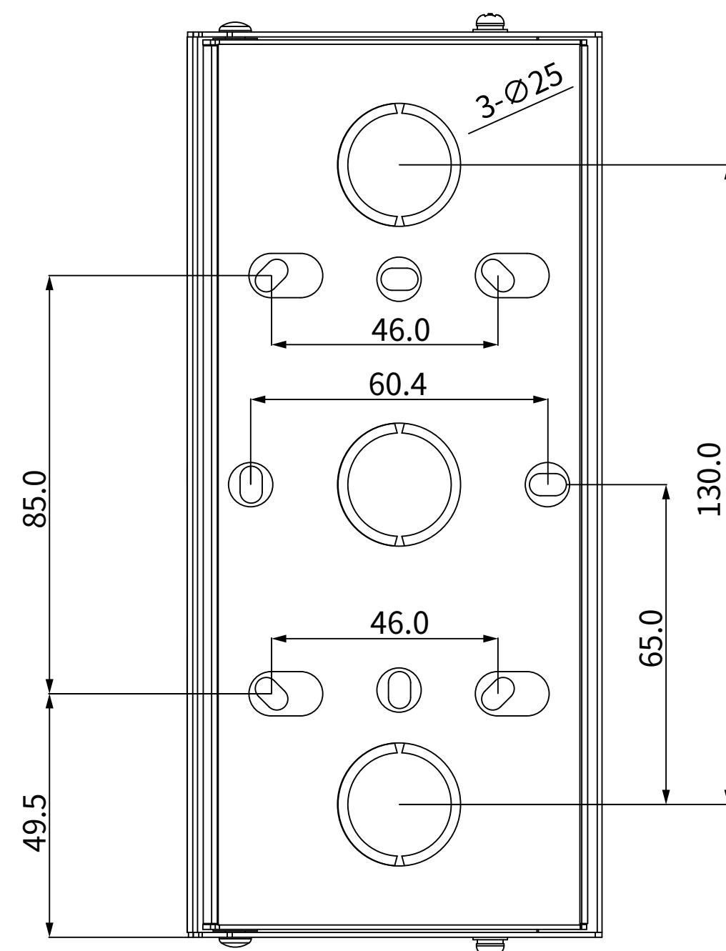
4 BACK VIEW
