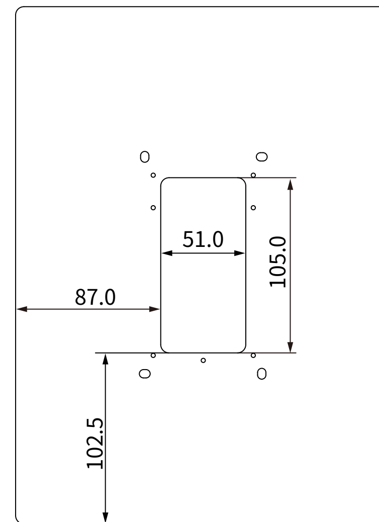
4 BACK VIEW
