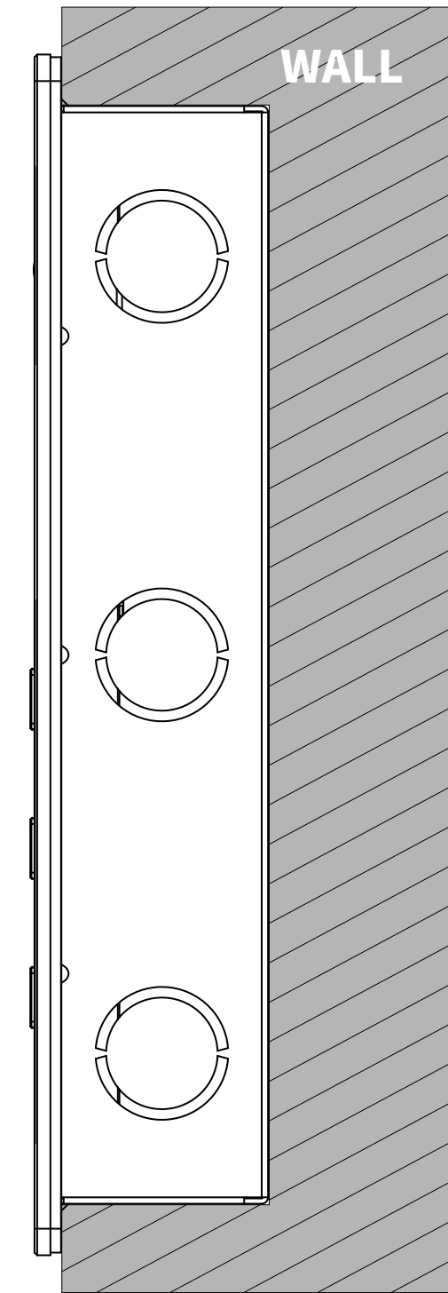
③ SIDE VIEW:INTERCOM PANEL IN WALL
