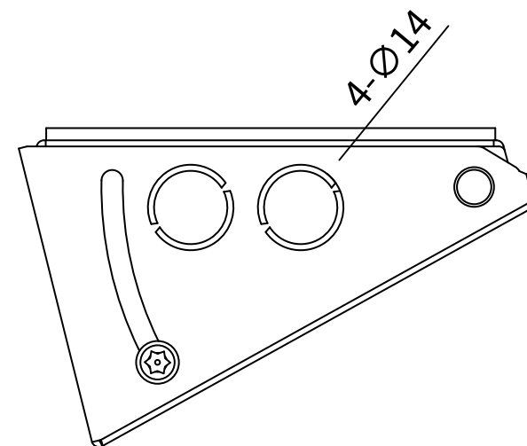
6 BOTTOM VIEW
