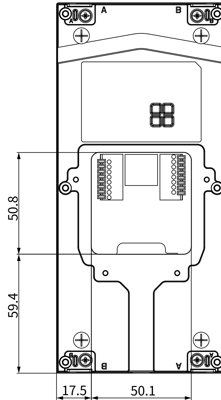
4 BACK VIEW
