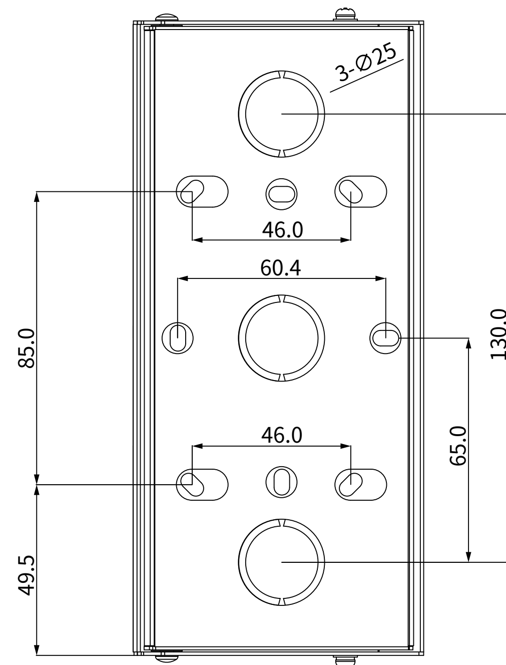
4 BACK VIEW
