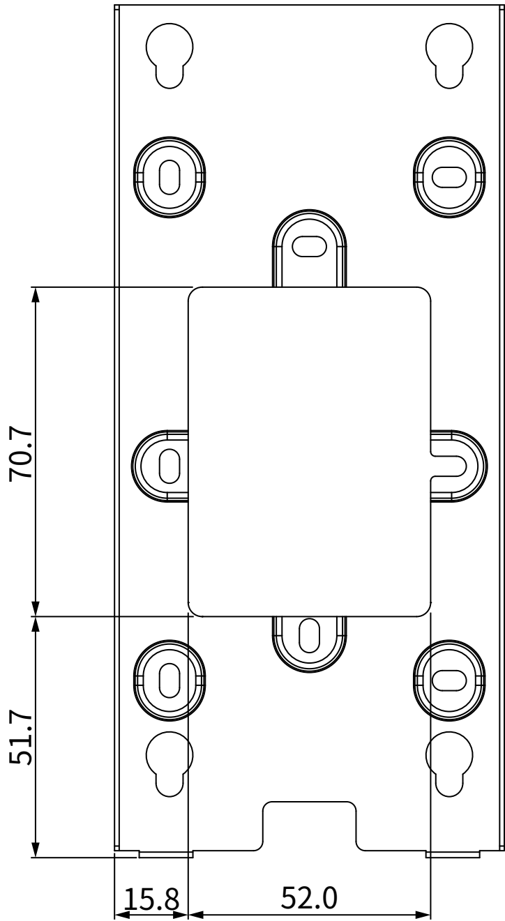
4 BACK VIEW
