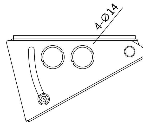
6 BOTTOM VIEW
