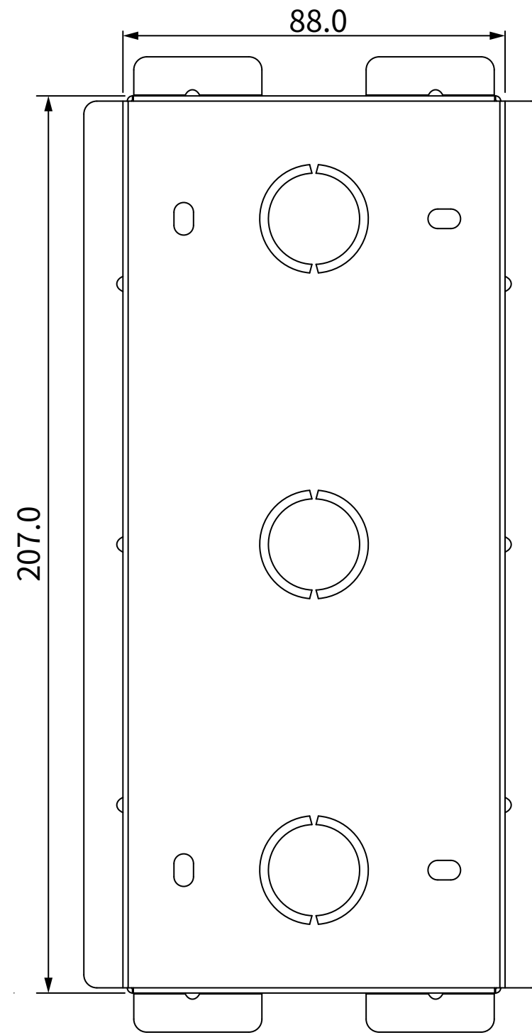
4 BACK VIEW
