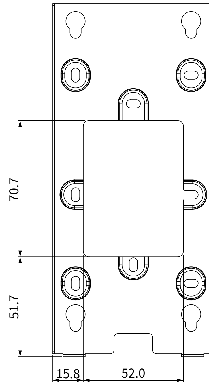
4 BACK VIEW
