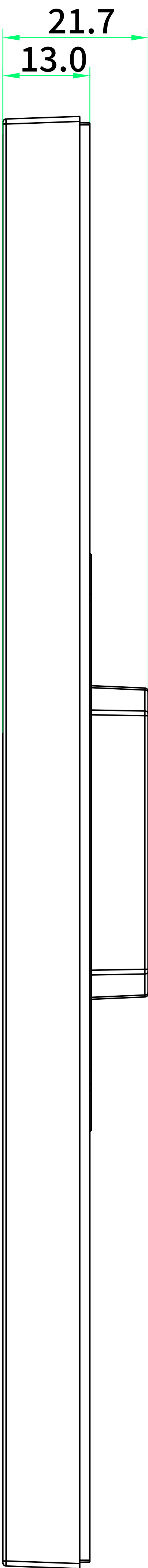
2 RIGHT VIEW
