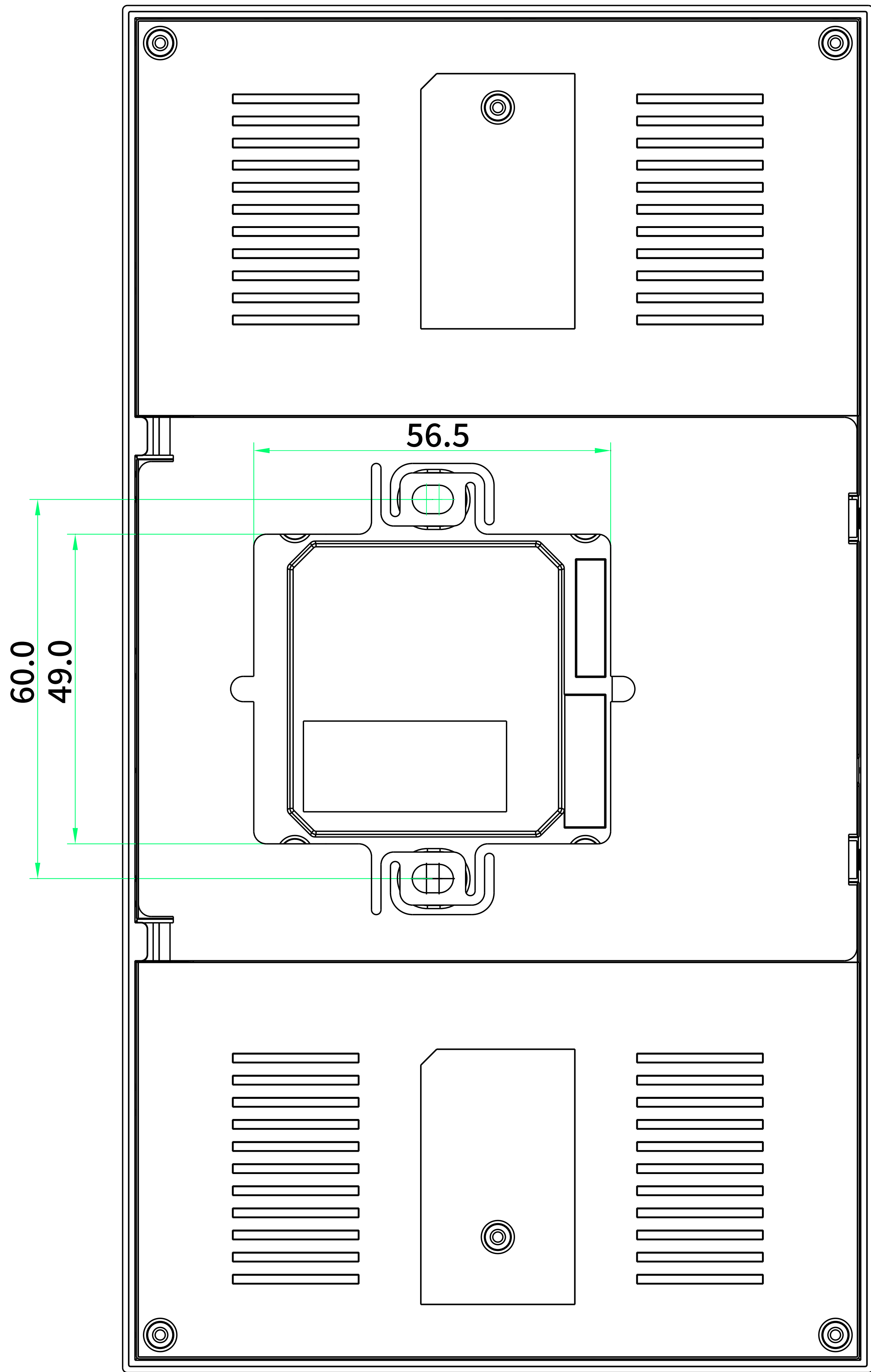
4 BACK VIEW
