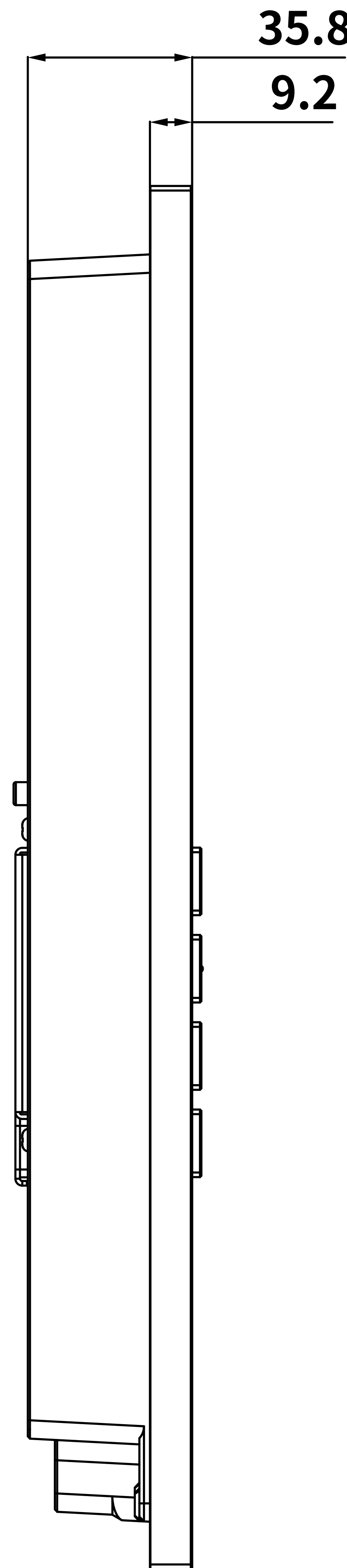
③ LEFT VIEW
