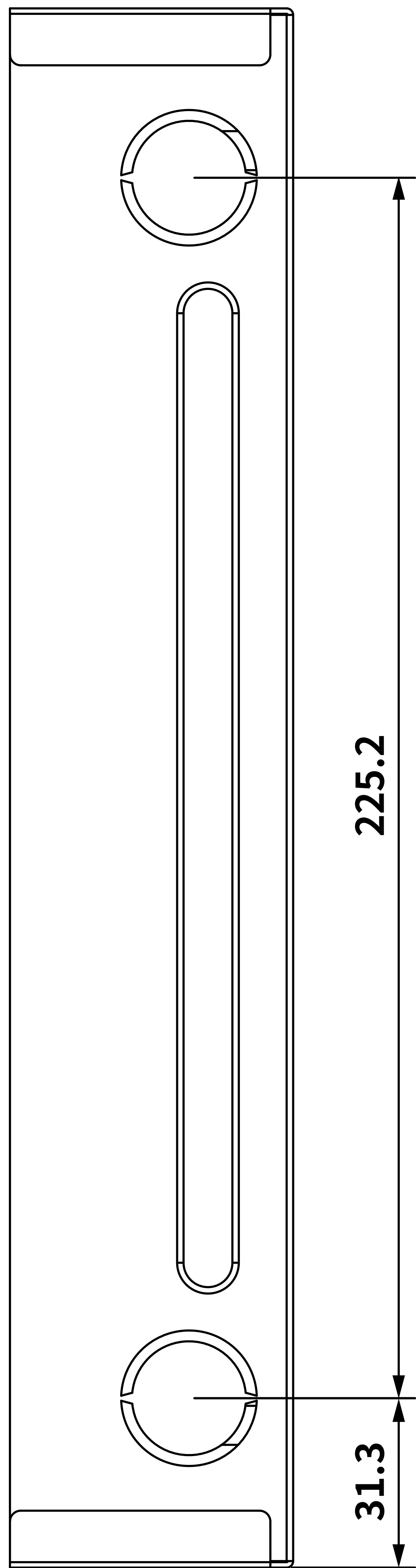
③ LEFT VIEW
