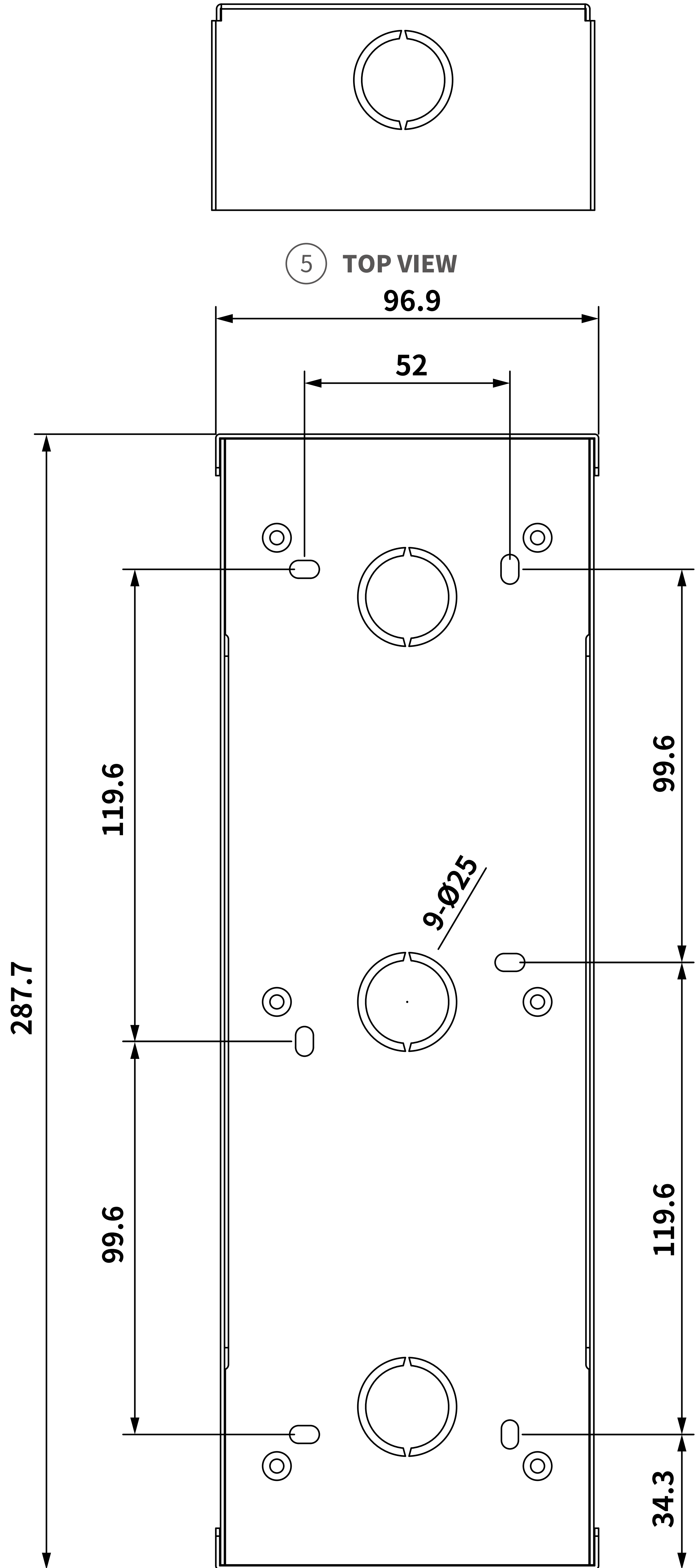
① FRONT VIEW
