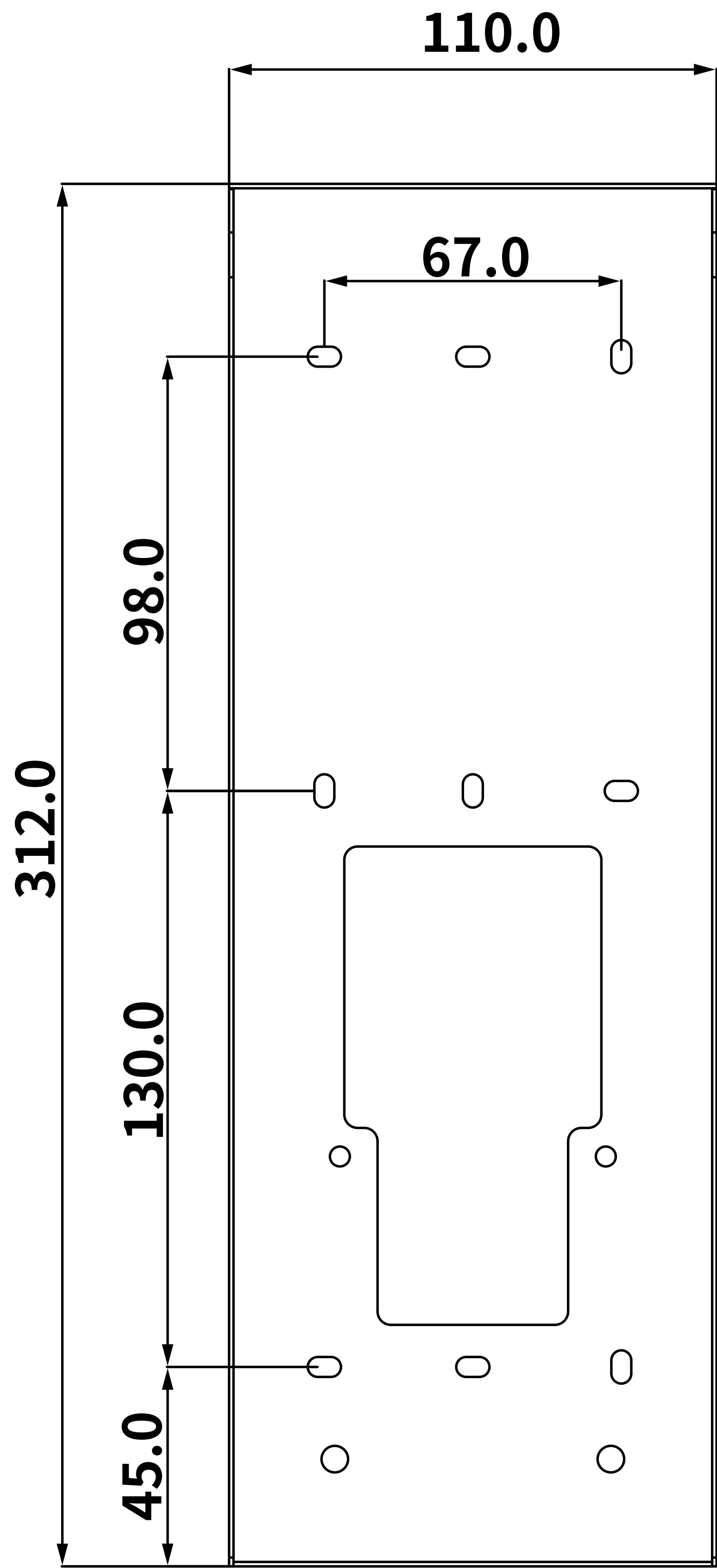
① FRONT VIEW
