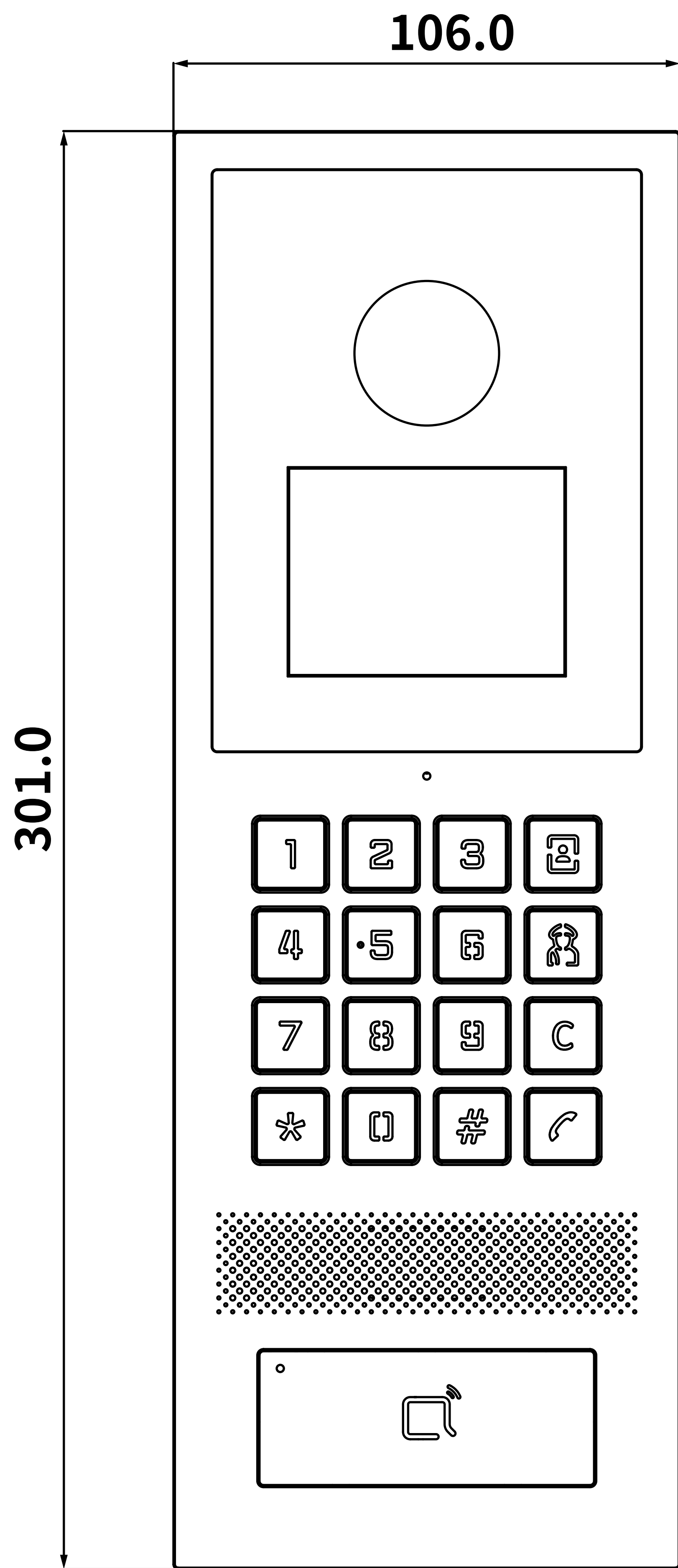
① FRONT VIEW
