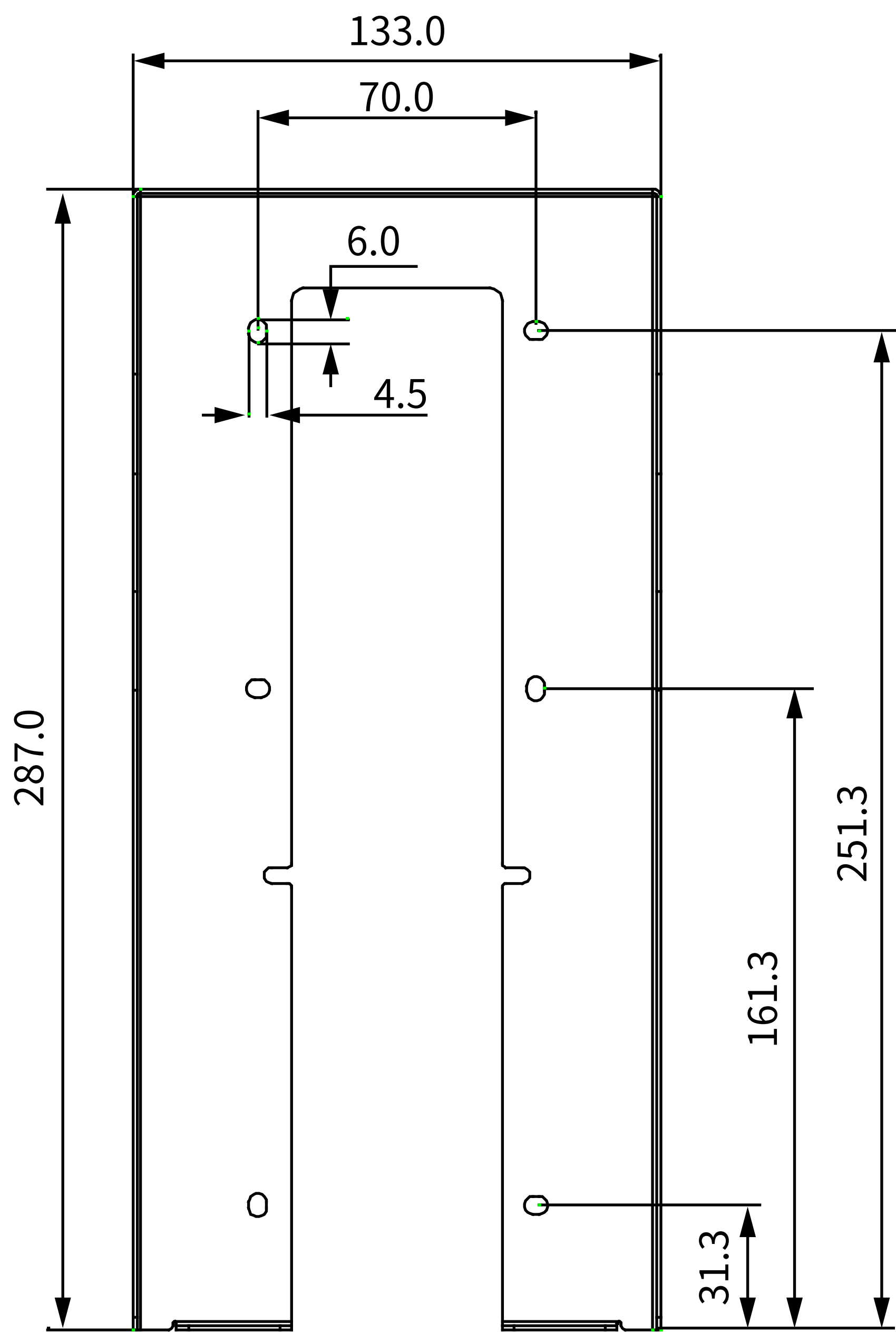
1 FRONT VIEW
