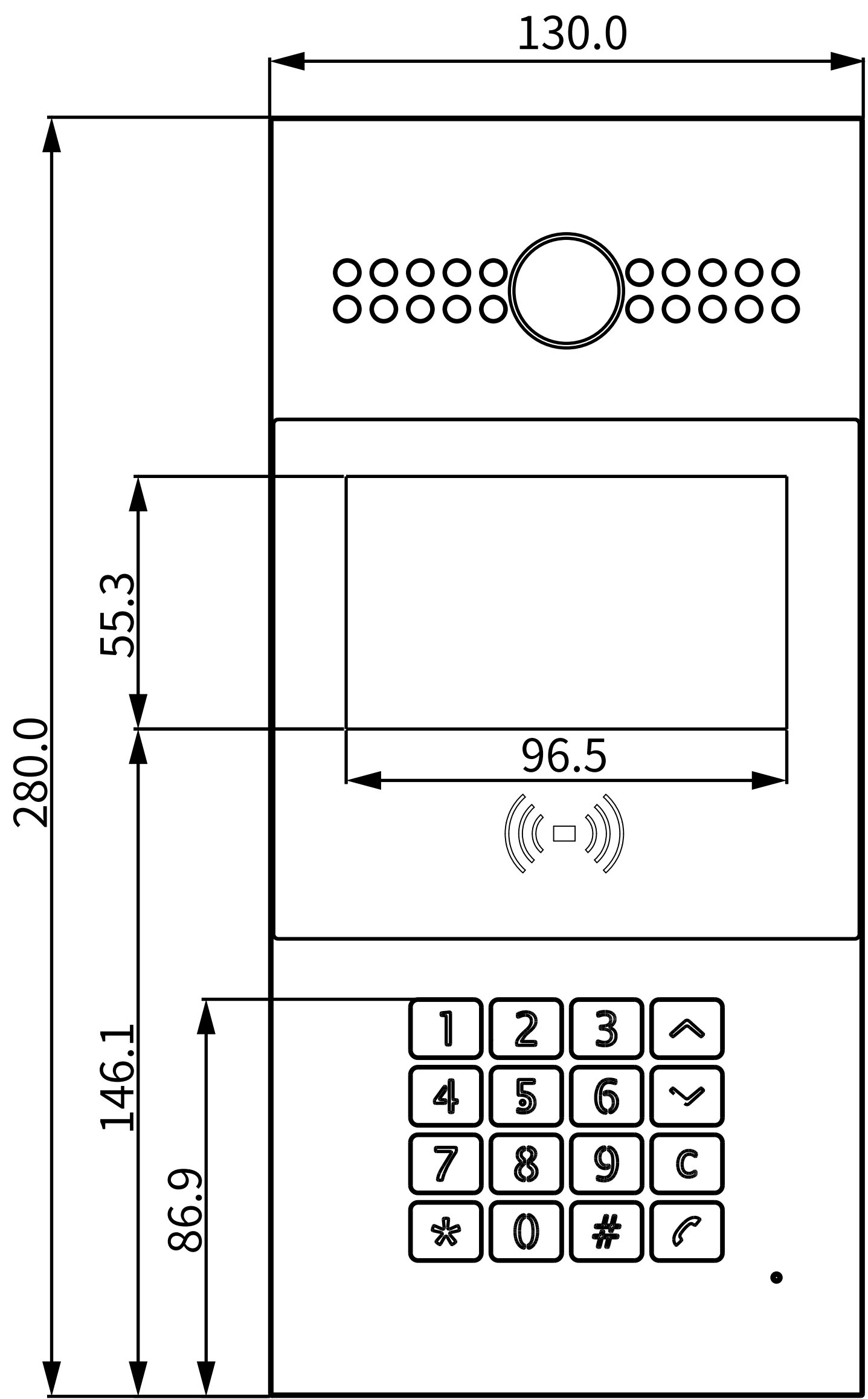
1 FRONT VIEW
