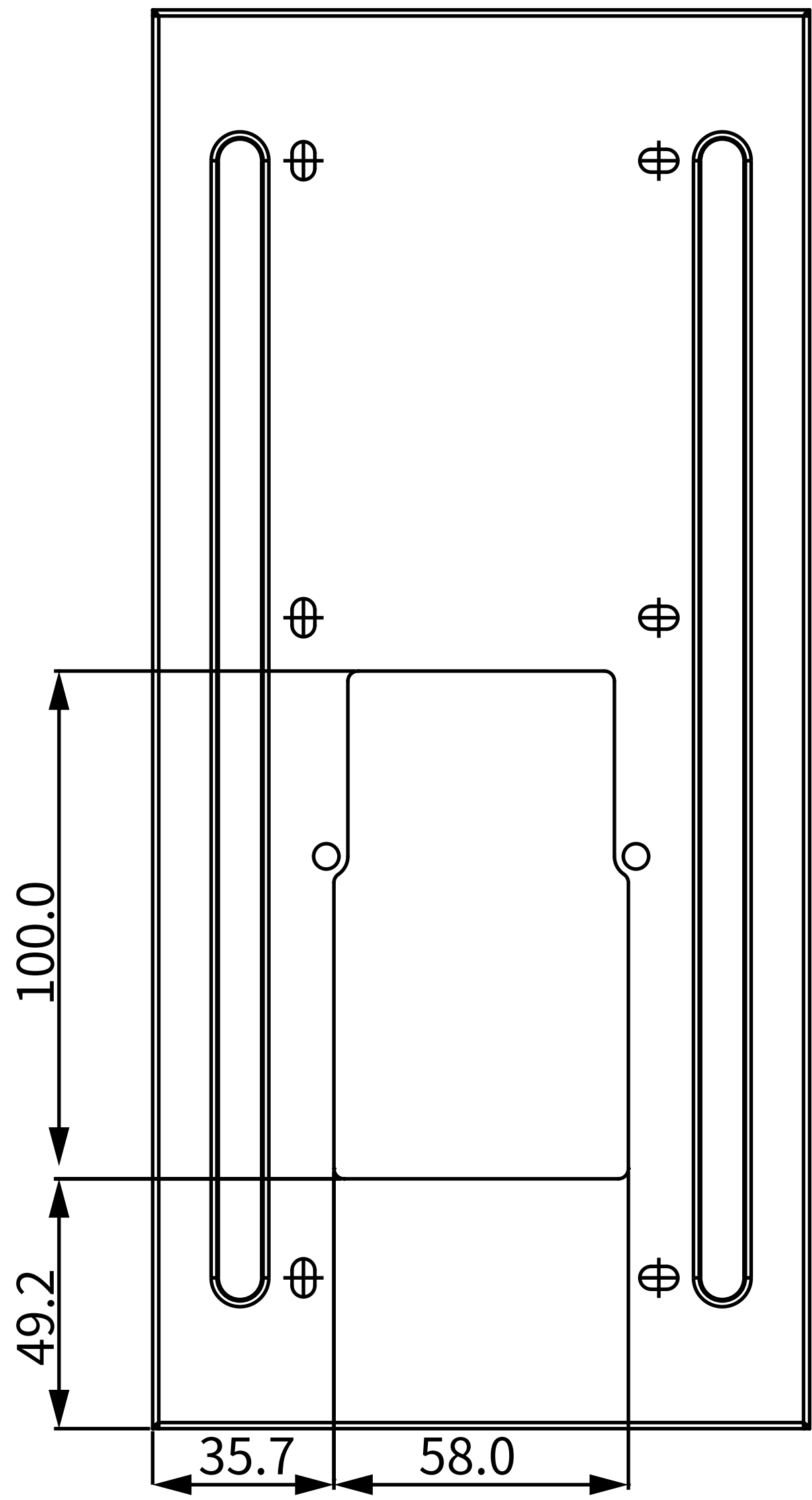
④ BACK VIEW
