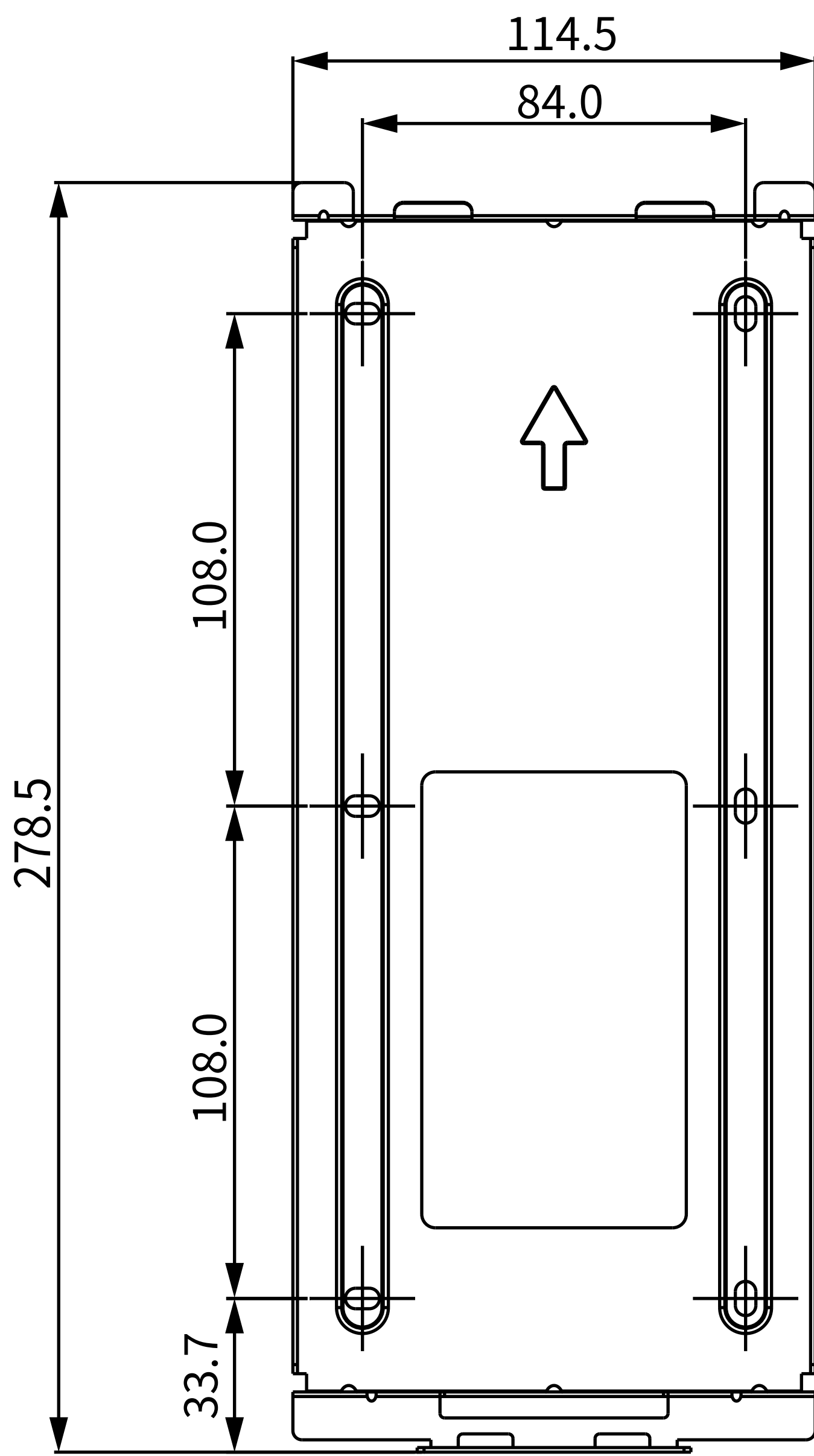
1 FRONT VIEW
