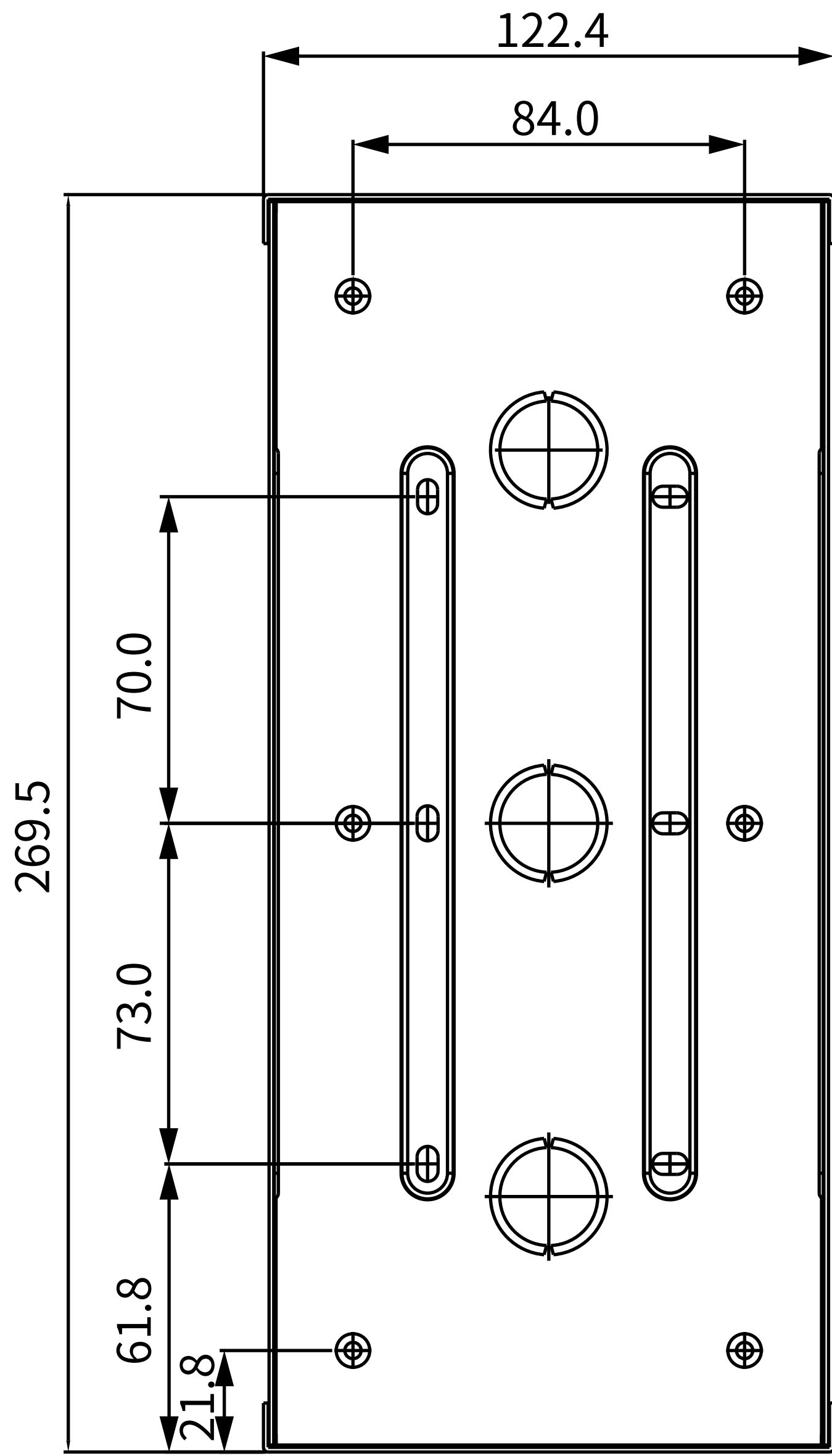
1 FRONT VIEW
