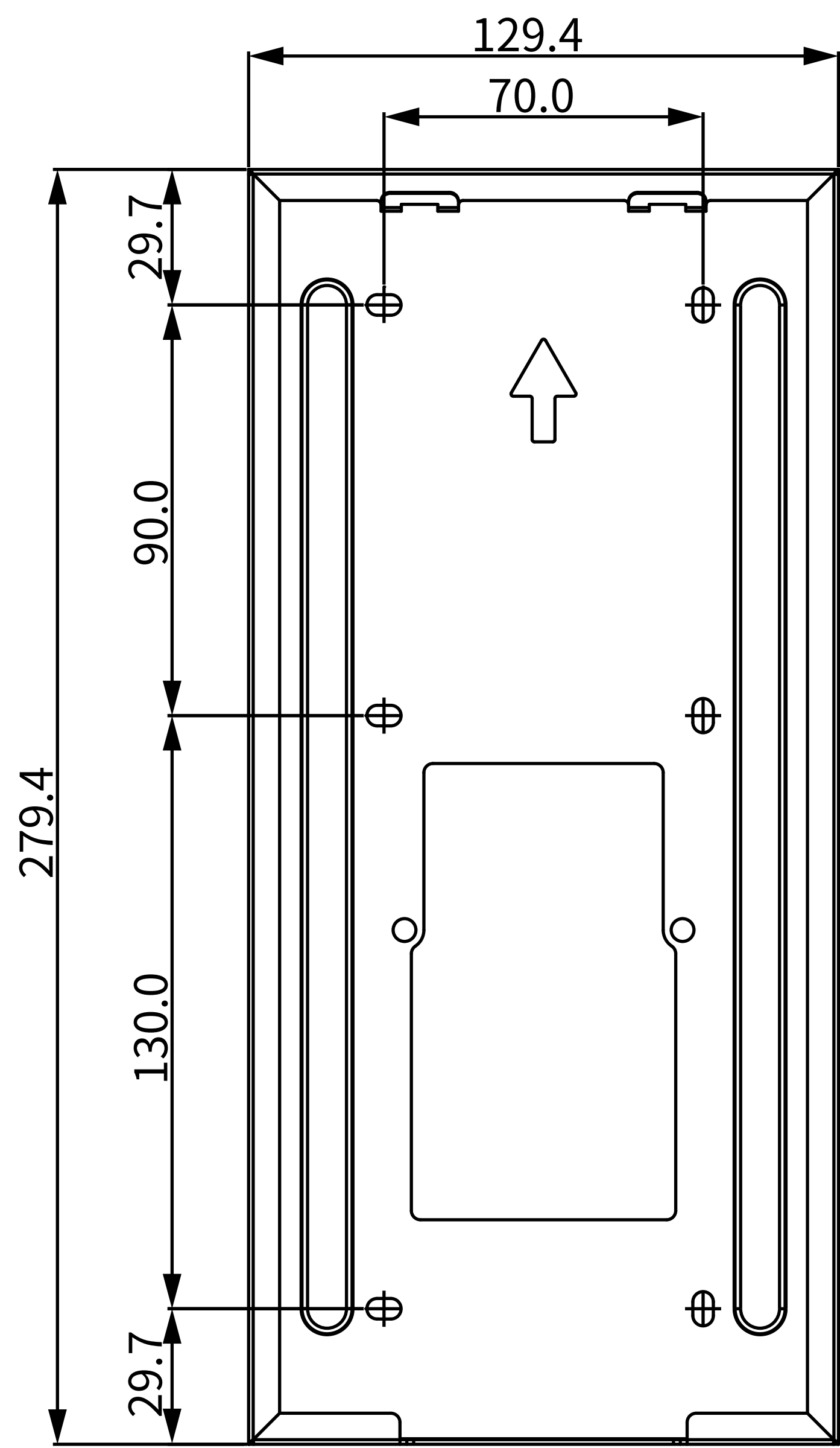
① FRONT VIEW
