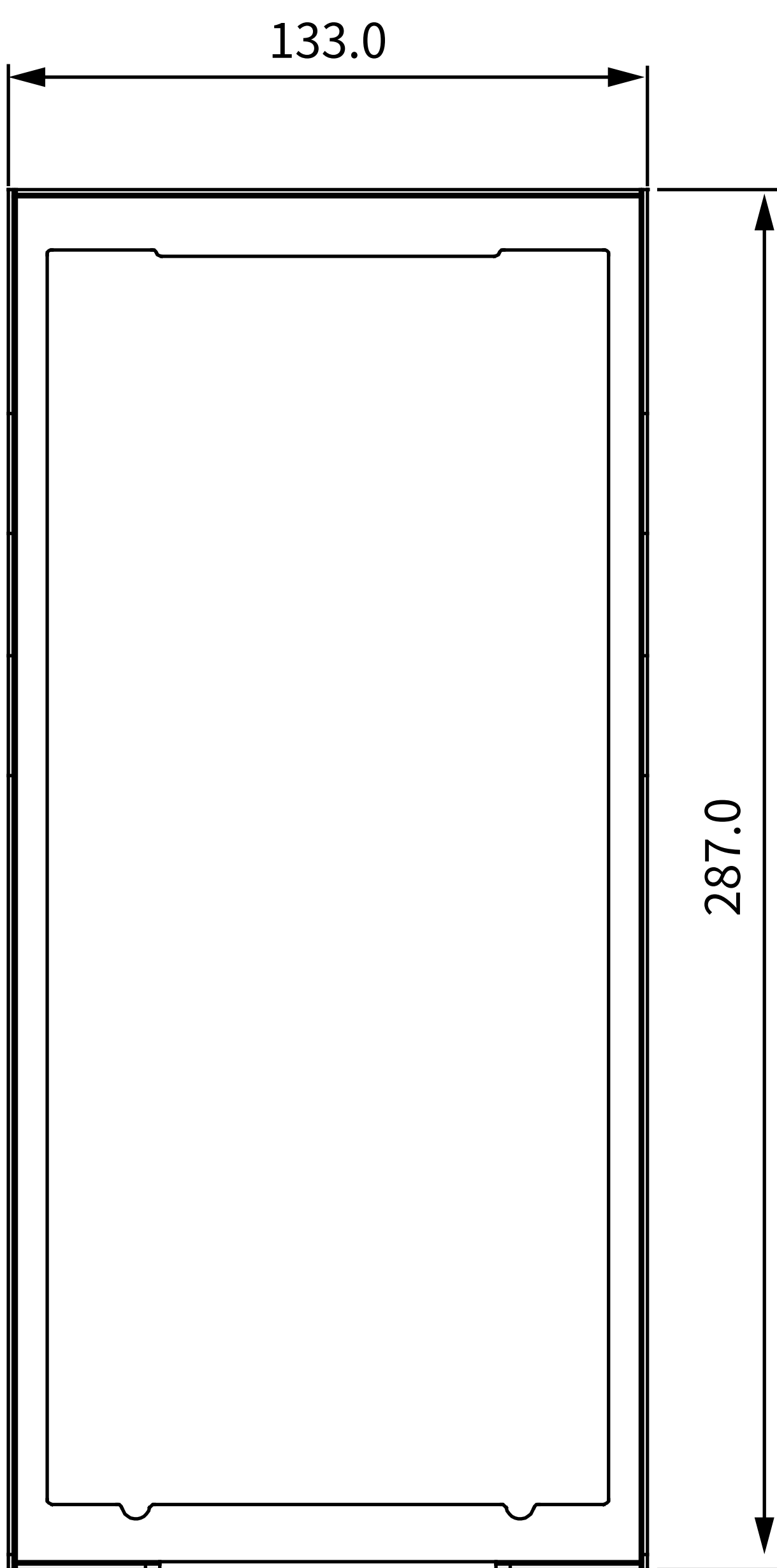
1 FRONT VIEW
