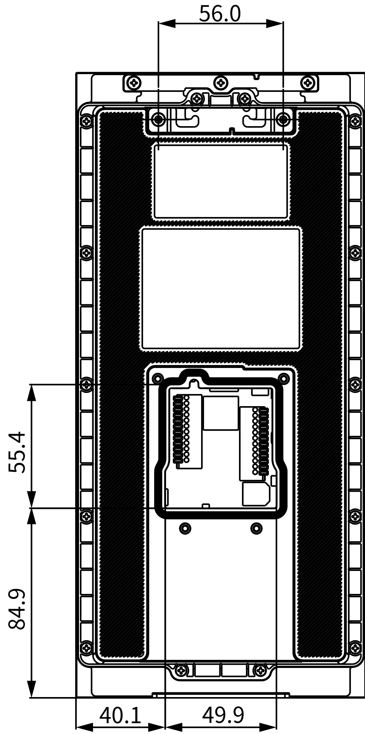
4 BACK VIEW
