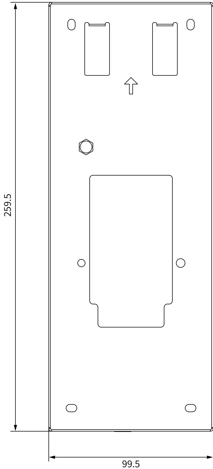
1 FRONT VIEW
