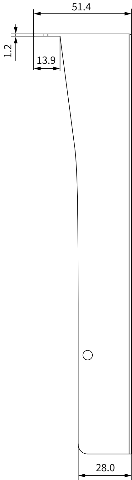
2 RIGHT VIEW
