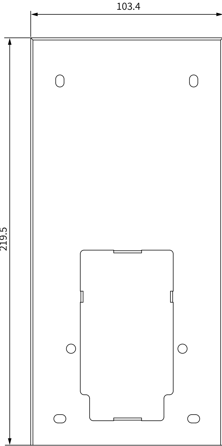
1 FRONT VIEW
