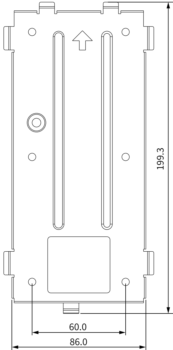
① FRONT VIEW
