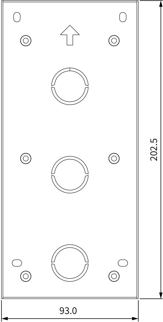
① FRONT VIEW
