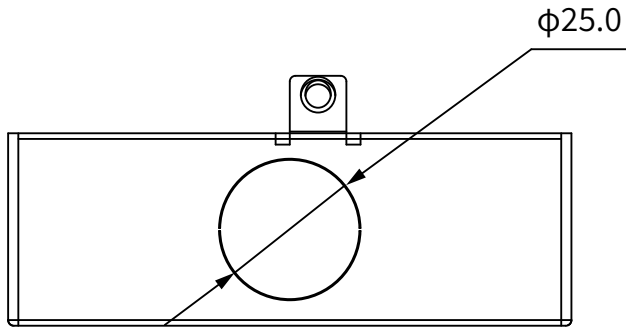
6 BOTTOM VIEW
