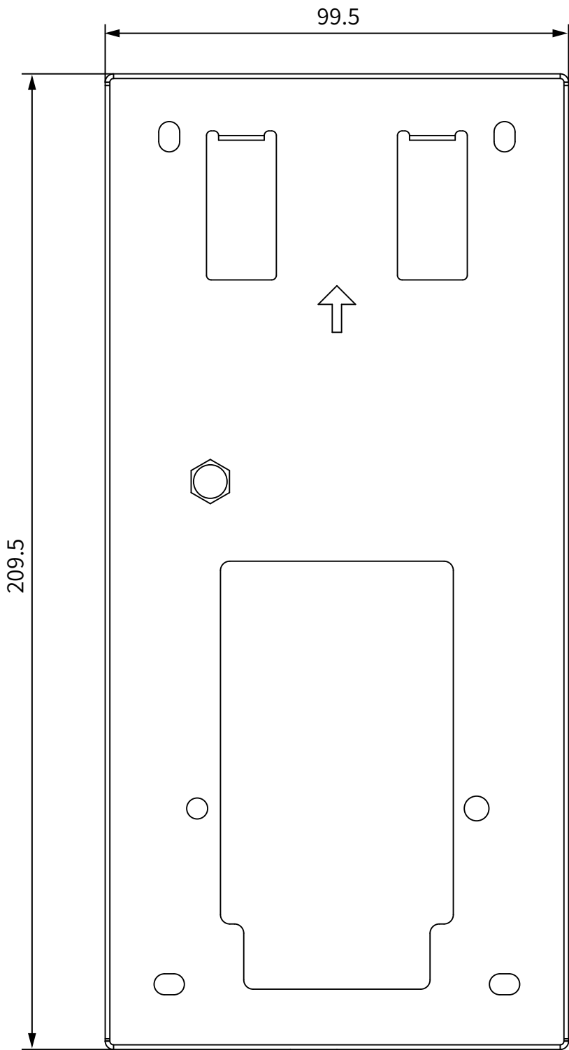
1 FRONT VIEW
