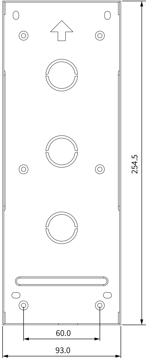
① FRONT VIEW
