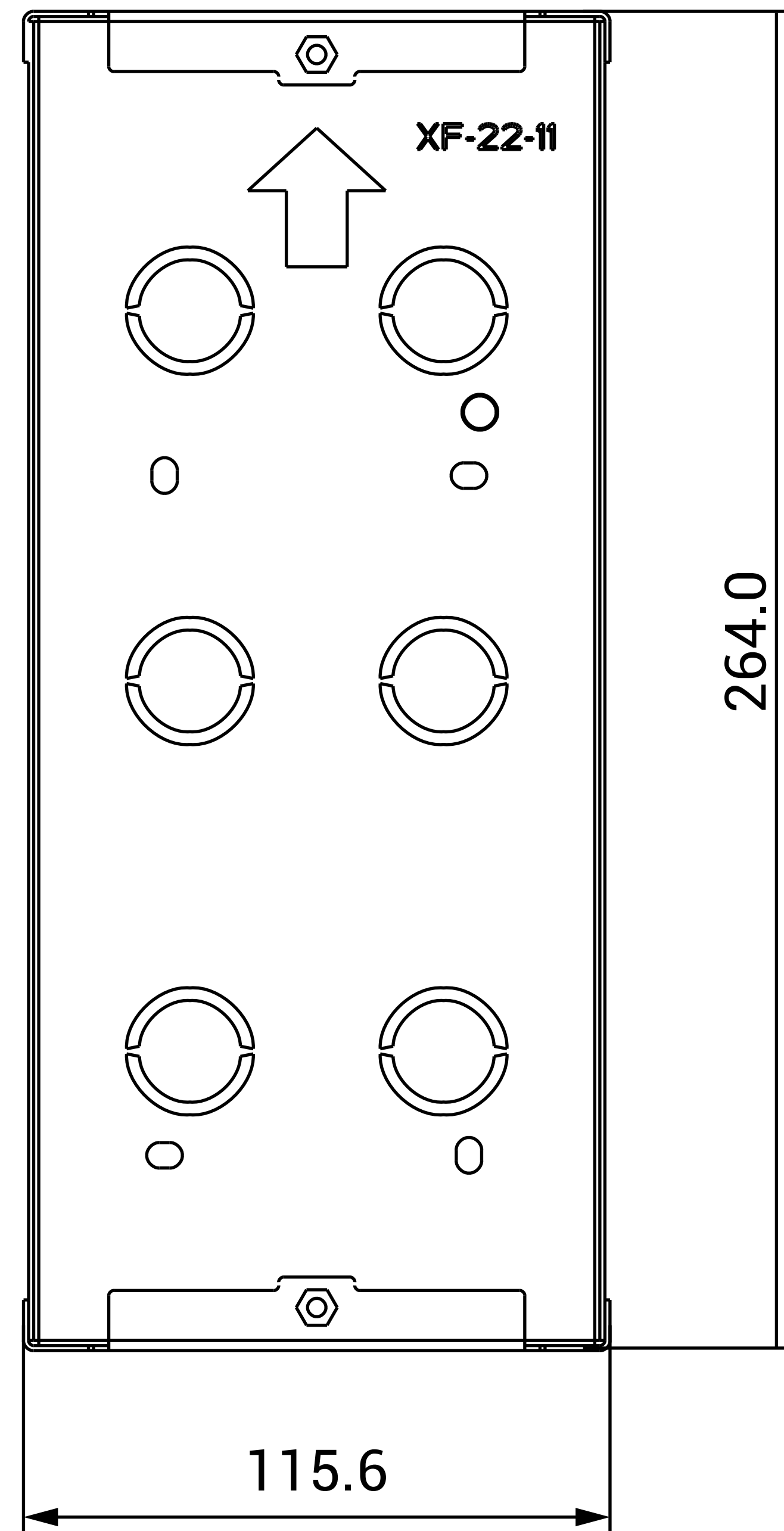
1 FRONT VIEW
