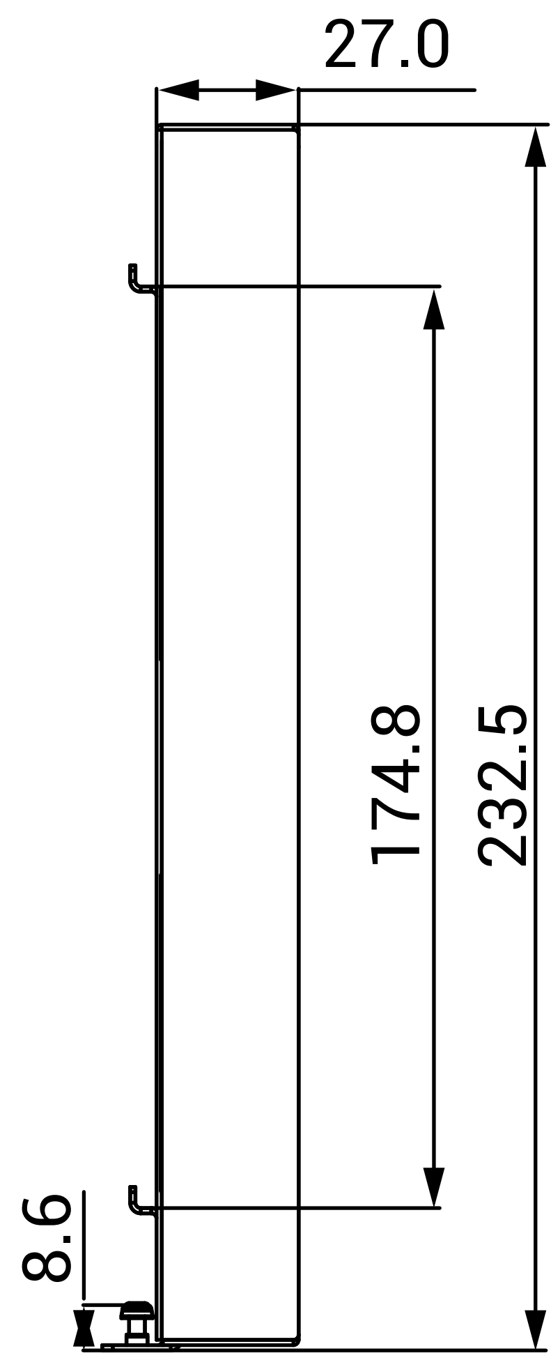
3 LEFT VIEW
