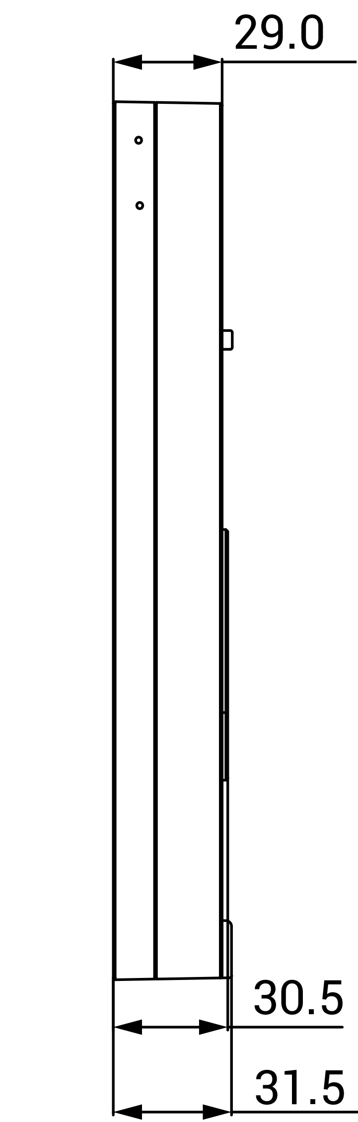
2 RIGHT VIEW
