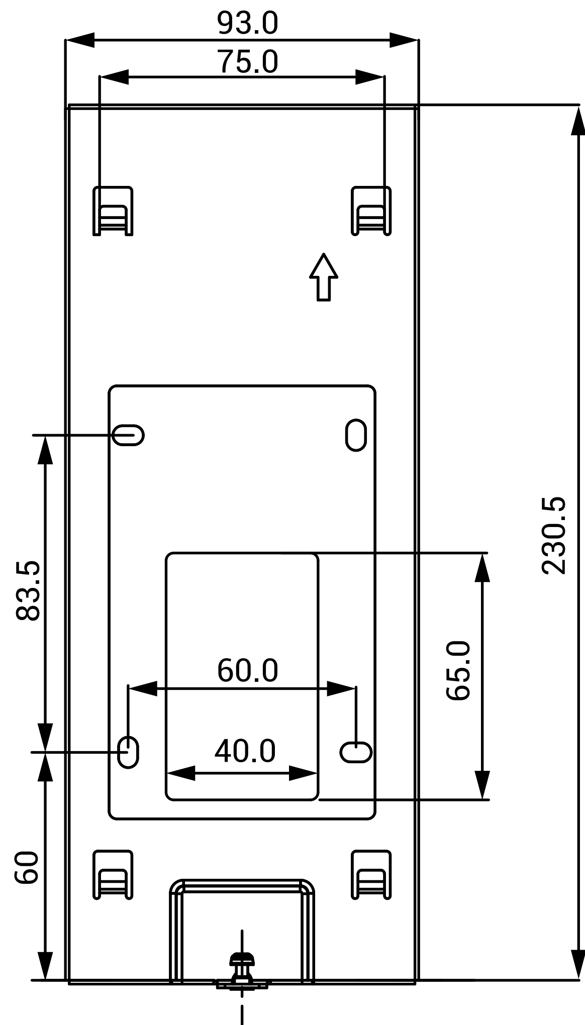
1 FRONT VIEW
