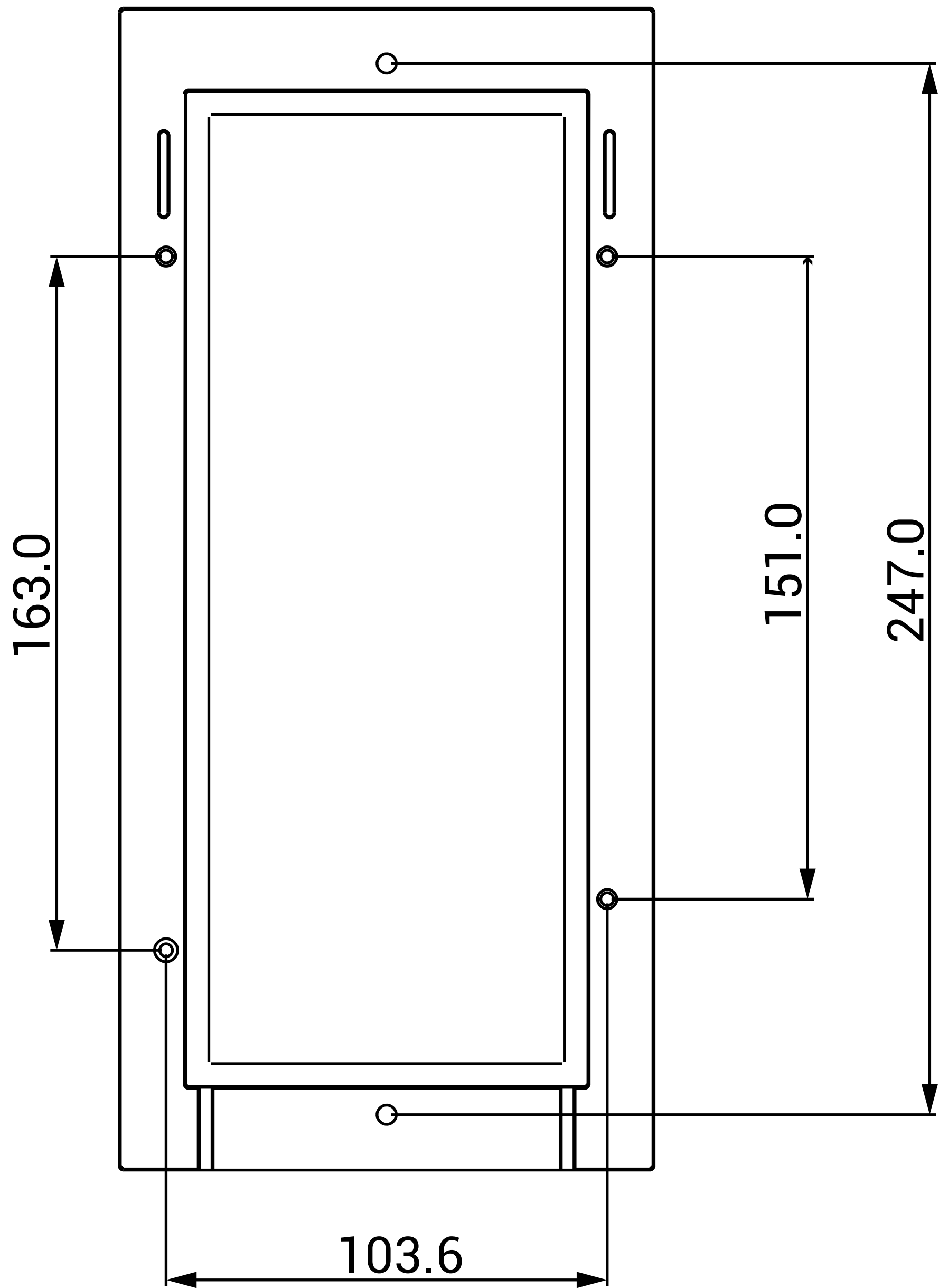
4 BACK VIEW
