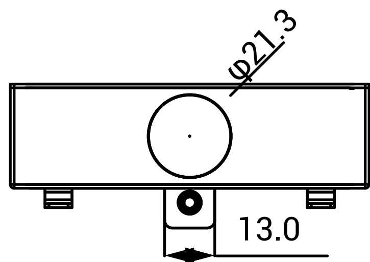
5 TOP VIEW
