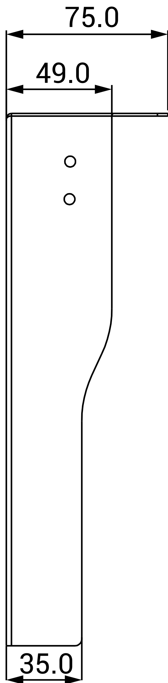
3 LEFT VIEW
