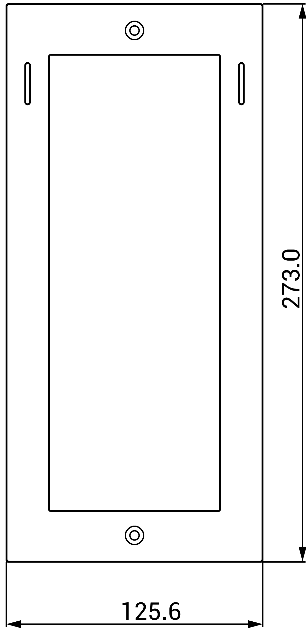
1 FRONT VIEW
