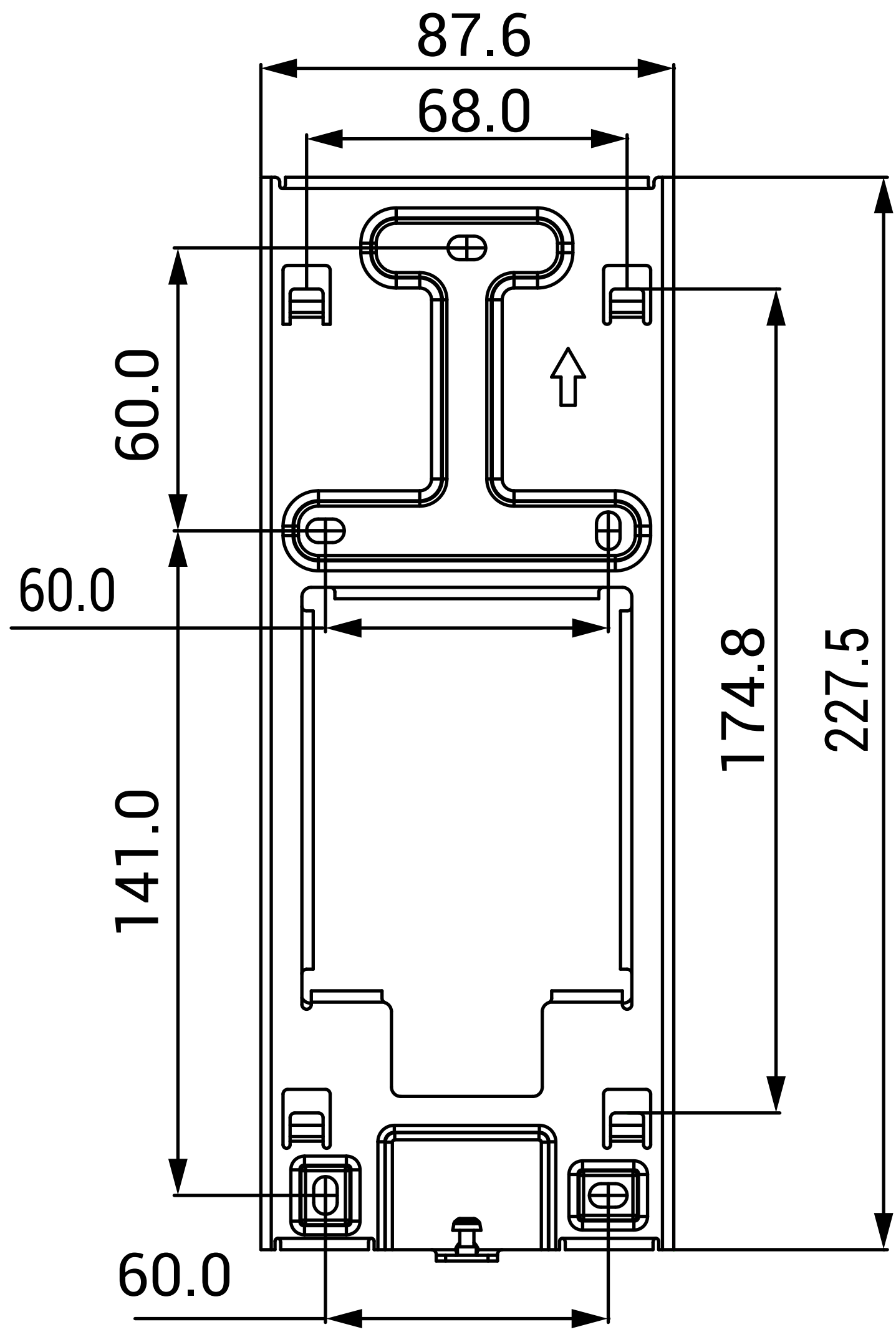
1 FRONT VIEW
