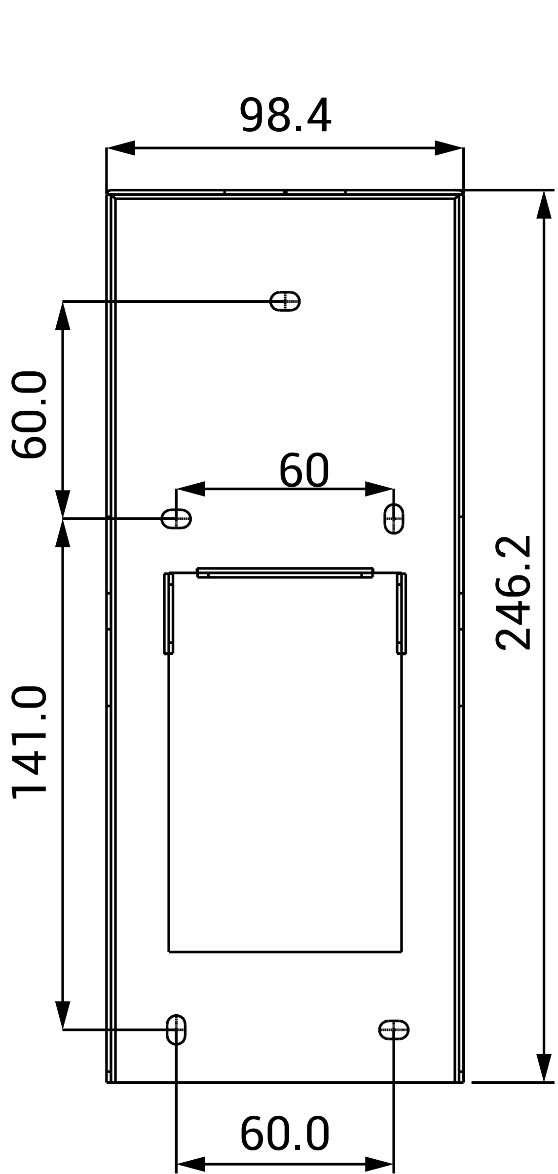
1 FRONT VIEW
