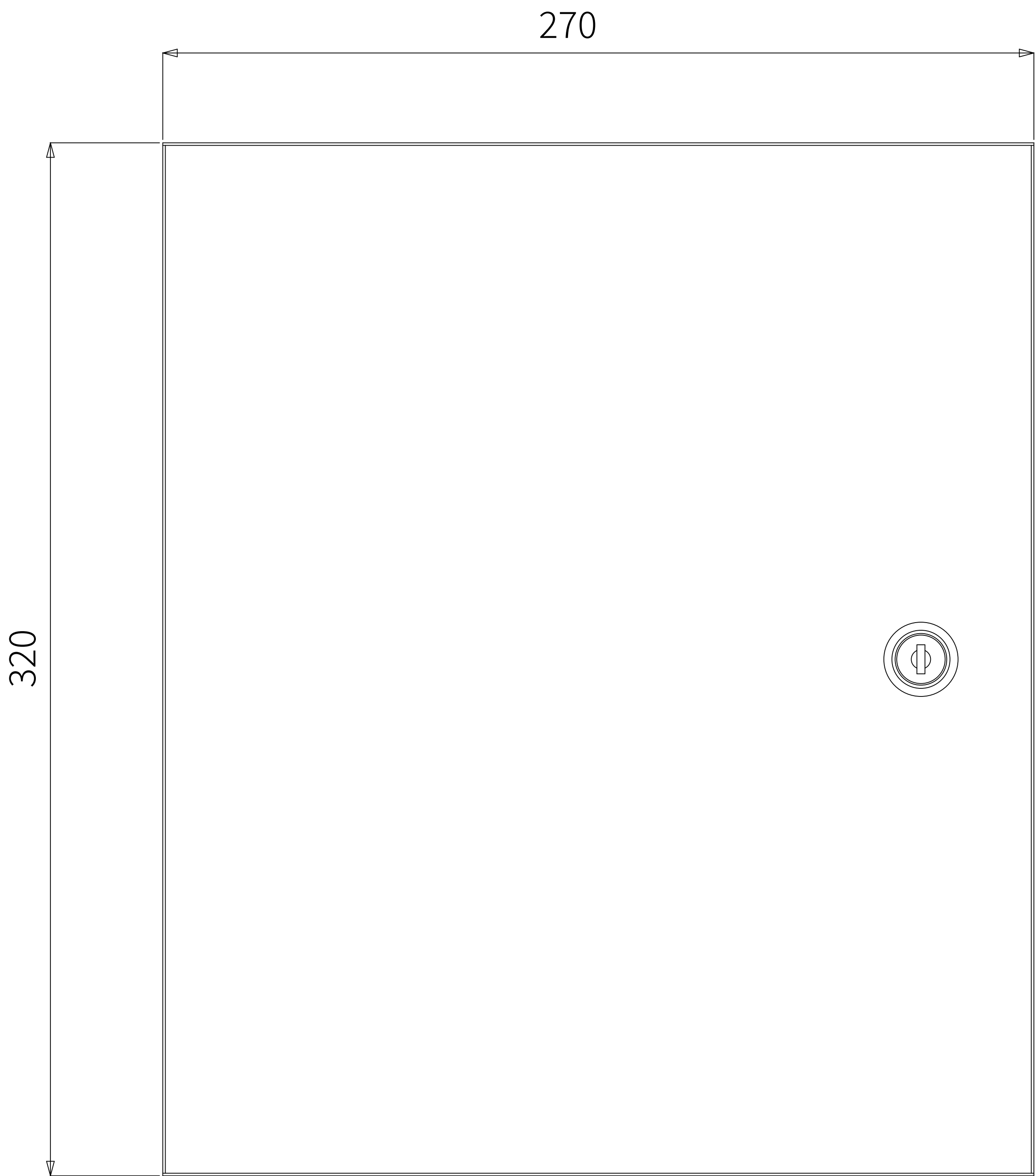
1 FRONT VIEW
