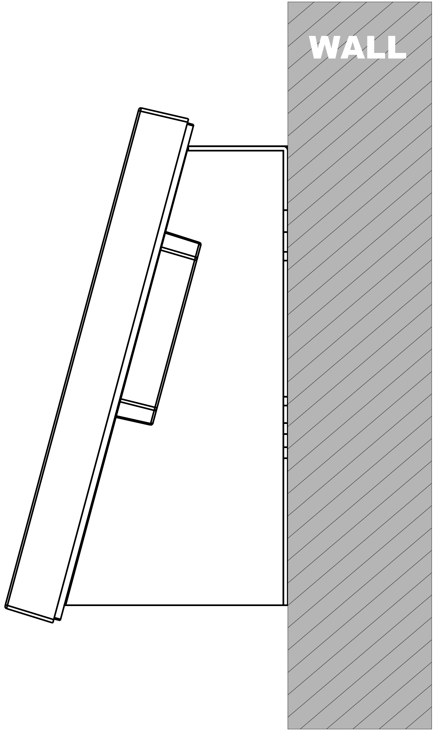
3 SIDE VIEW:INDOOR MONITOR ON WALL
