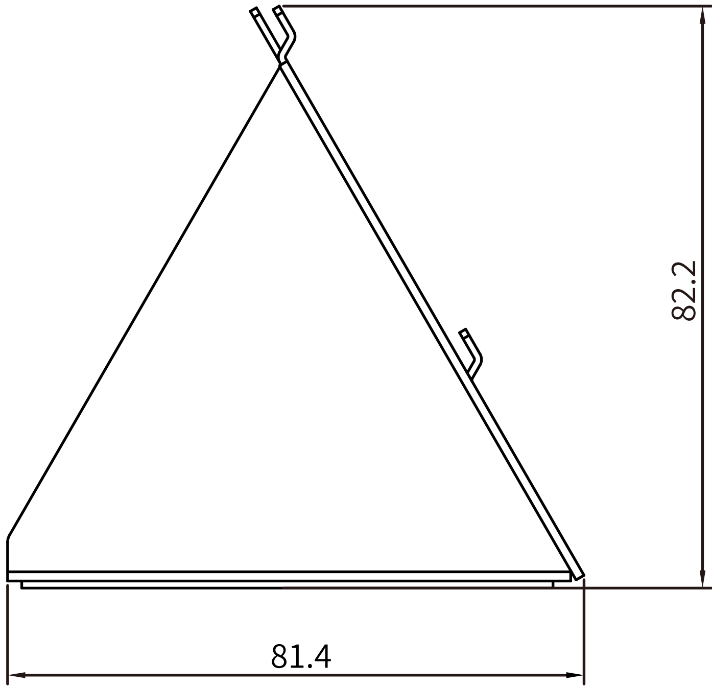
3 LEFT VIEW
