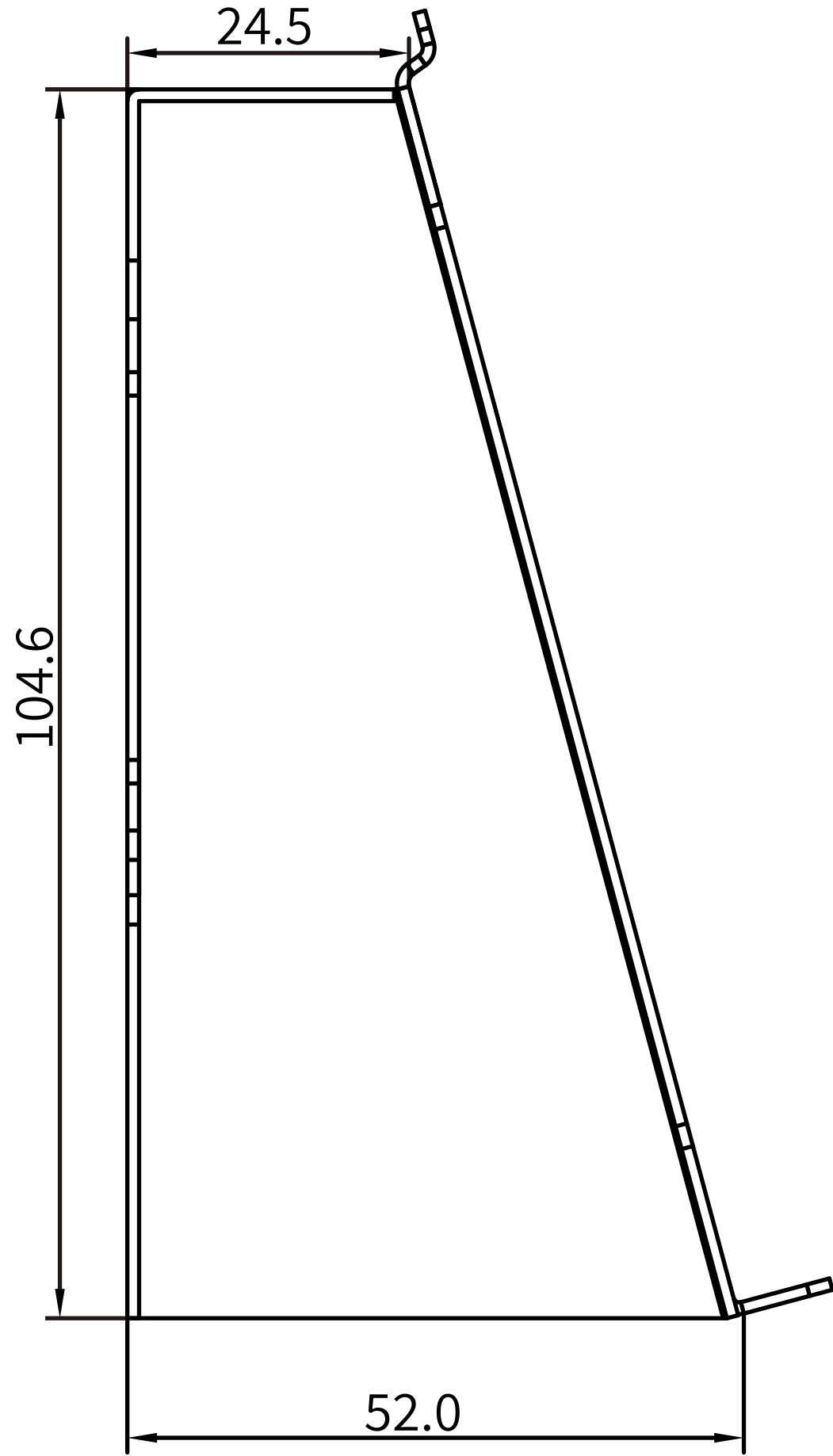
2 RIGHT VIEW
