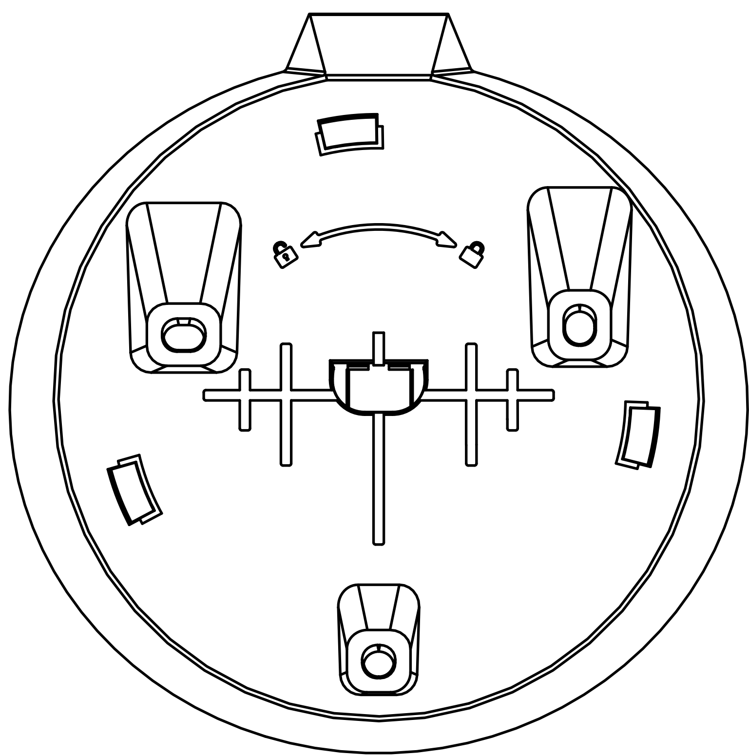
2 FRONT VIEW:WALL MOUNTING BRACKET
