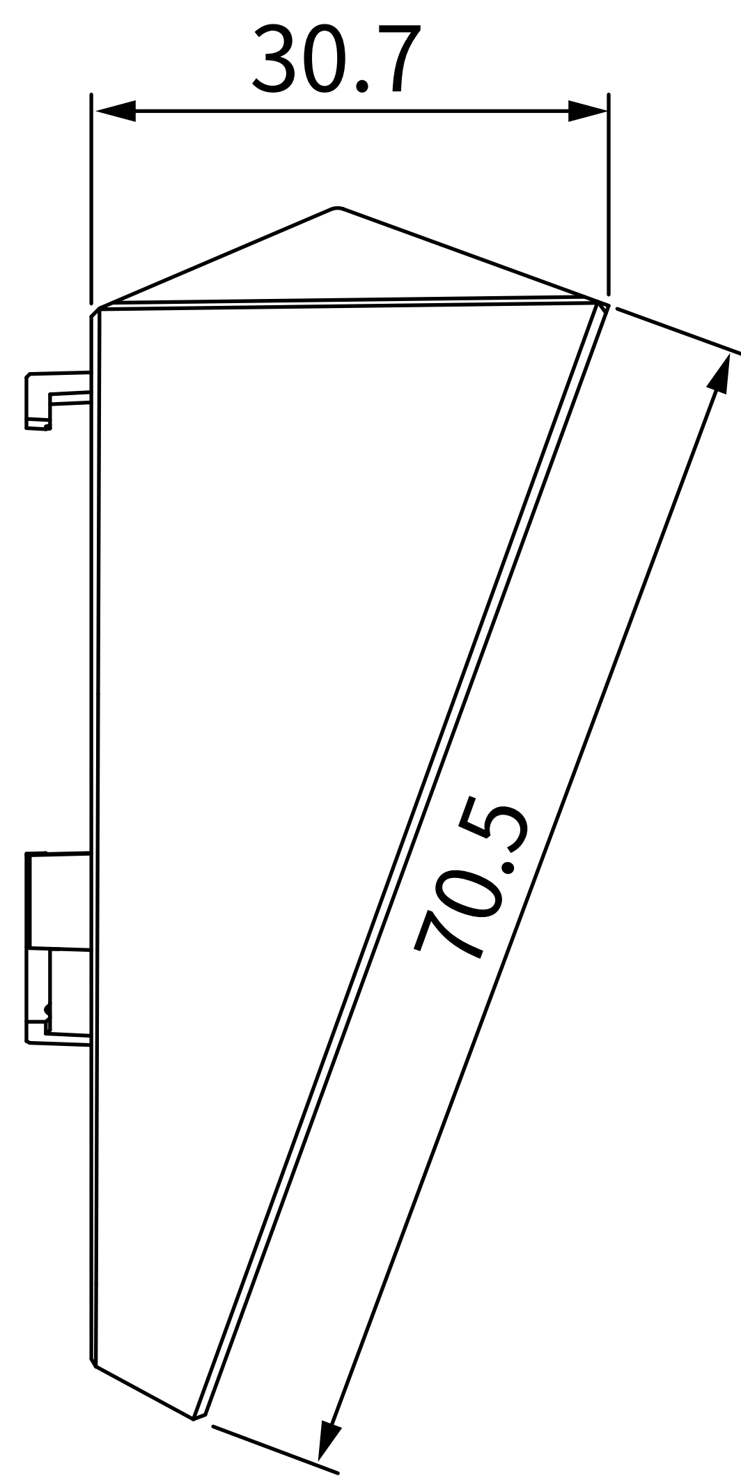
2 RIGHT VIEW
