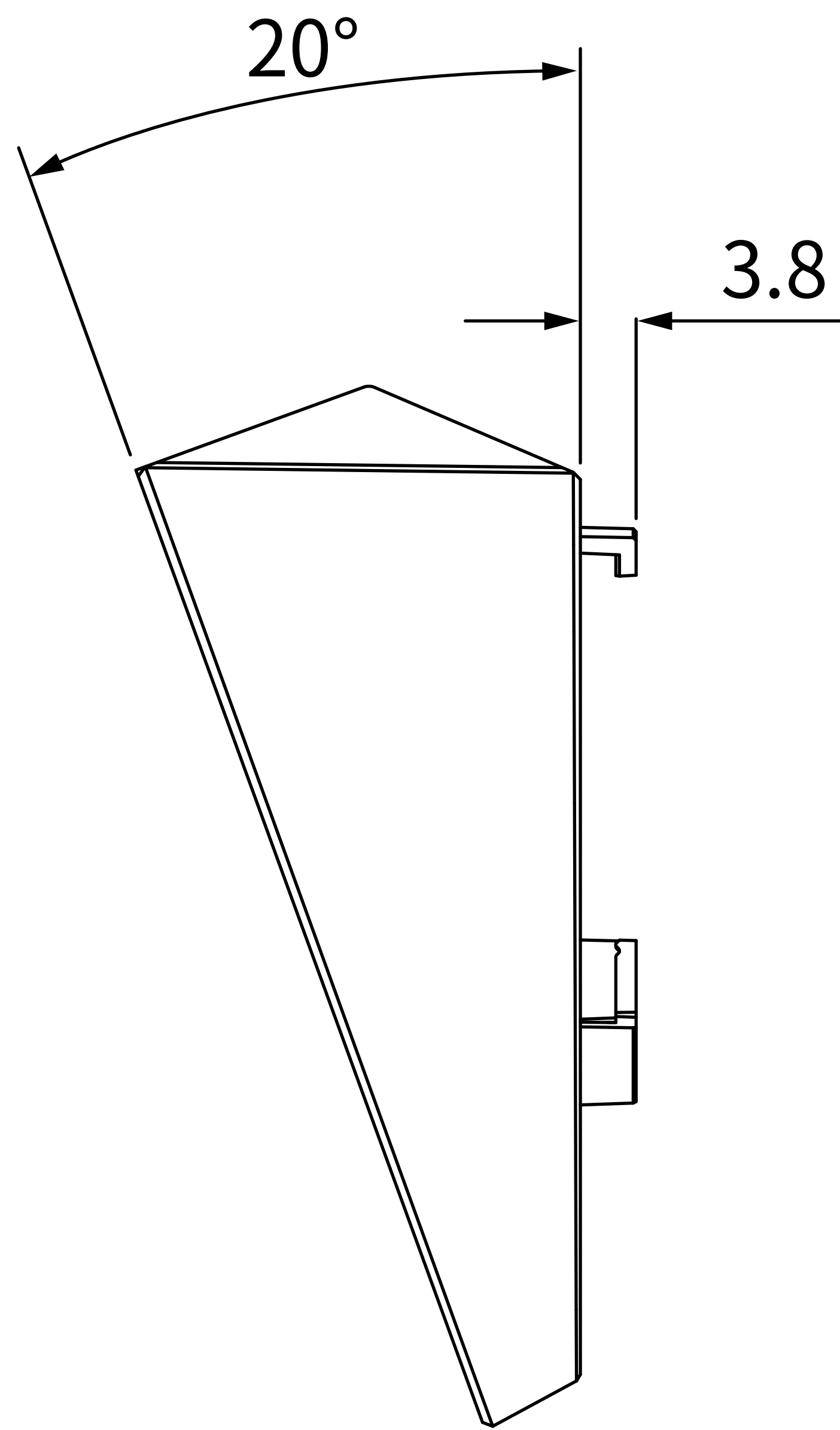
3 LEFT VIEW
