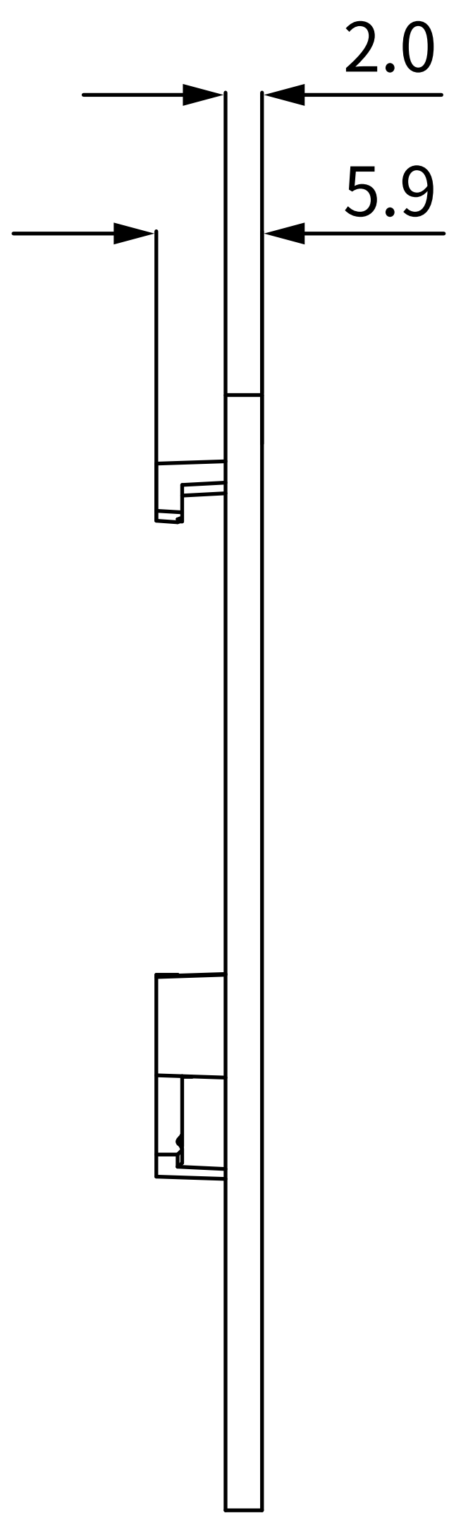
2 RIGHT VIEW
