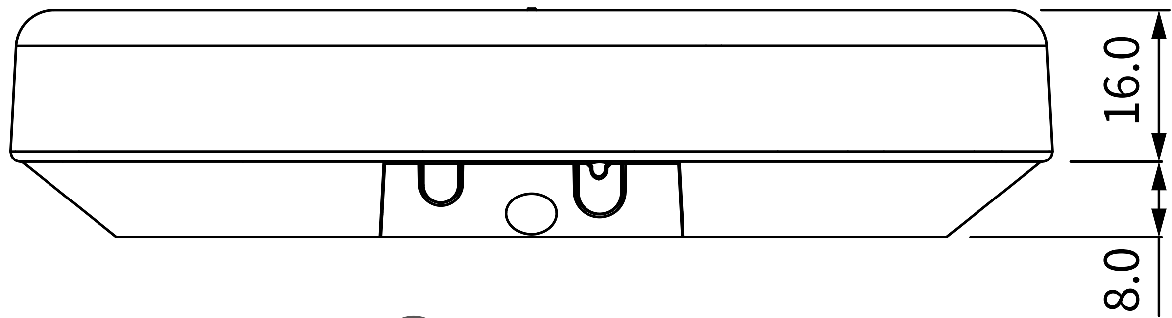
6 BOTTOM VIEW
