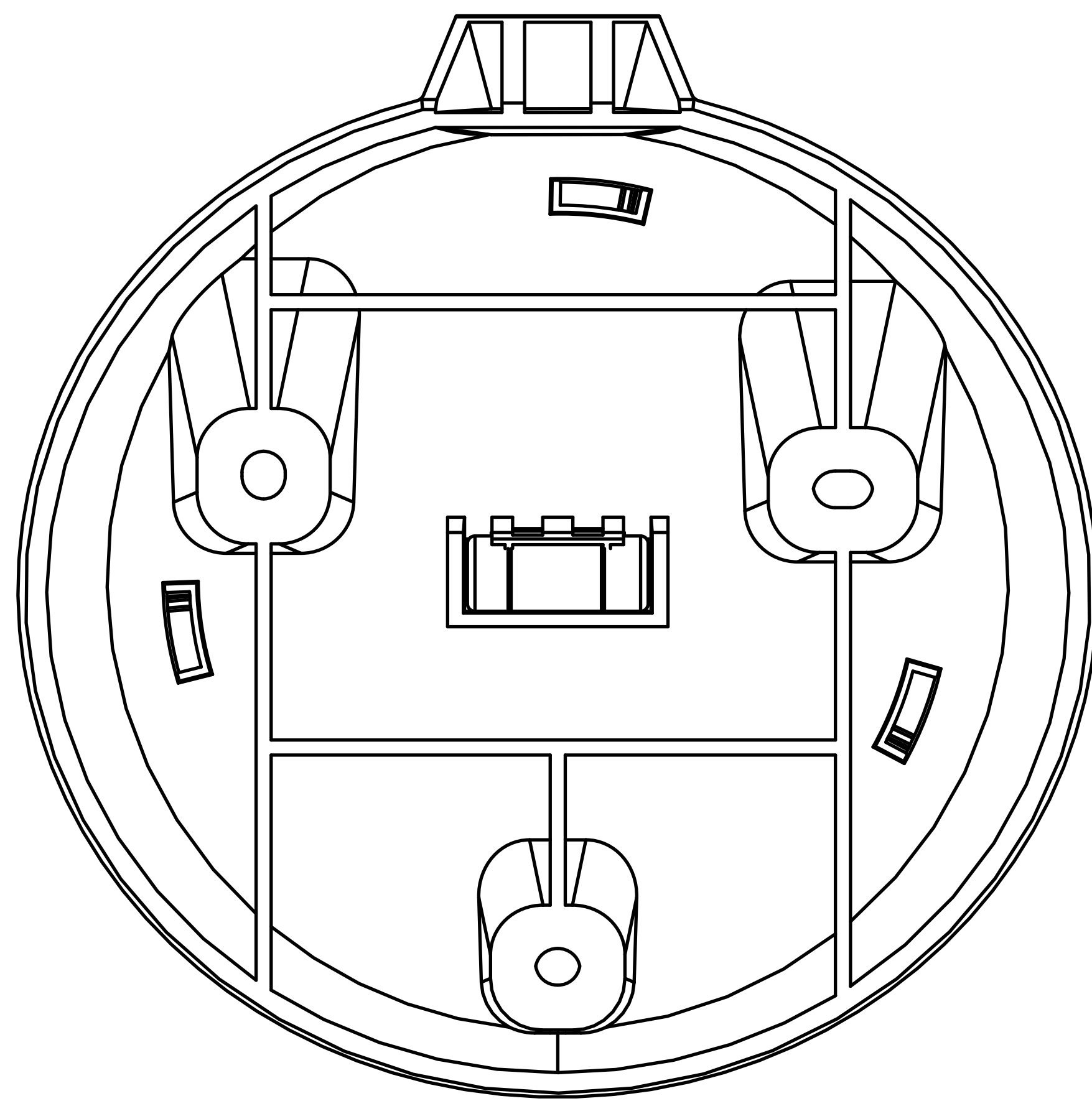
4 BACK VIEW
