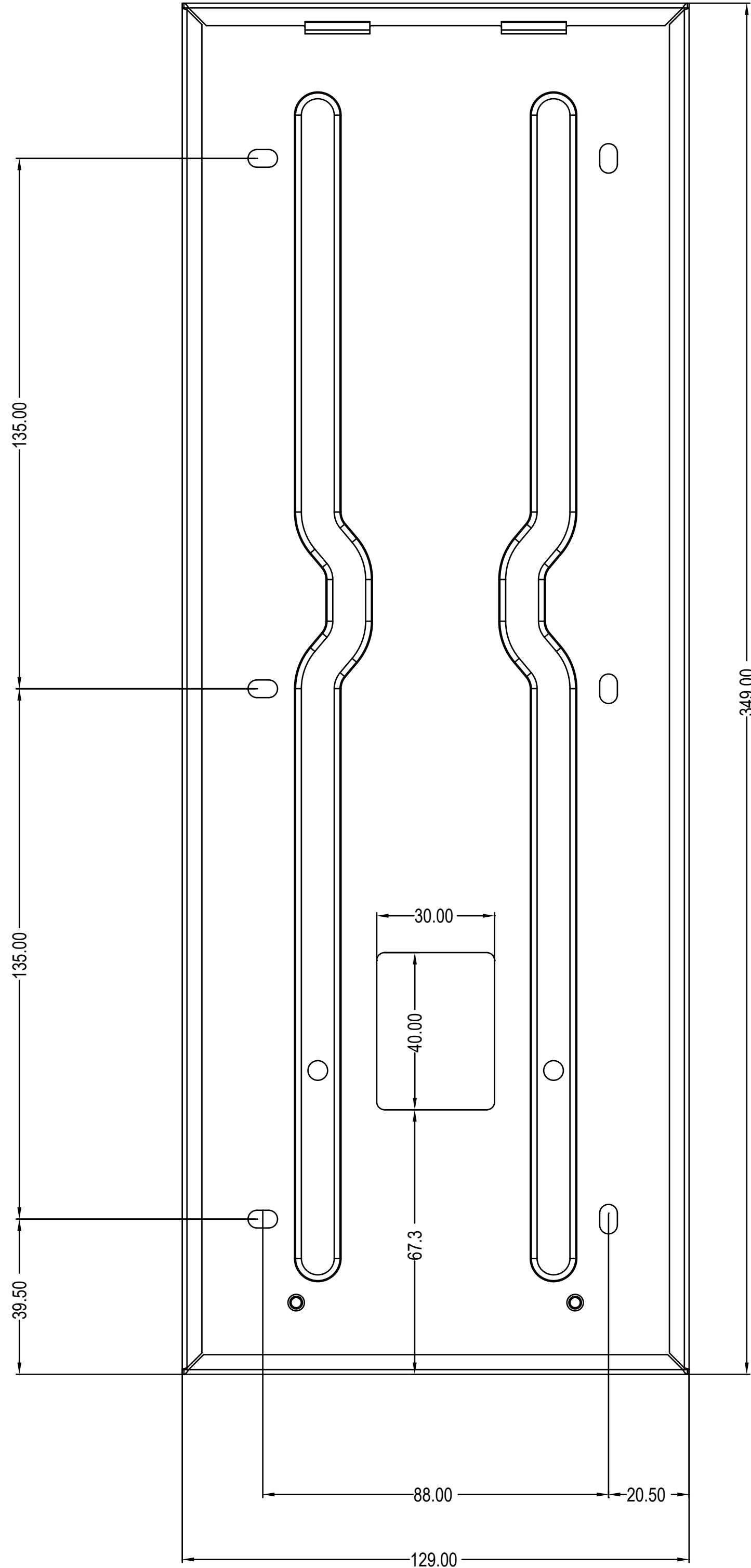
1 FRONT VIEW
