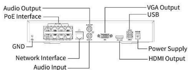
[NVR-108B-P8]
