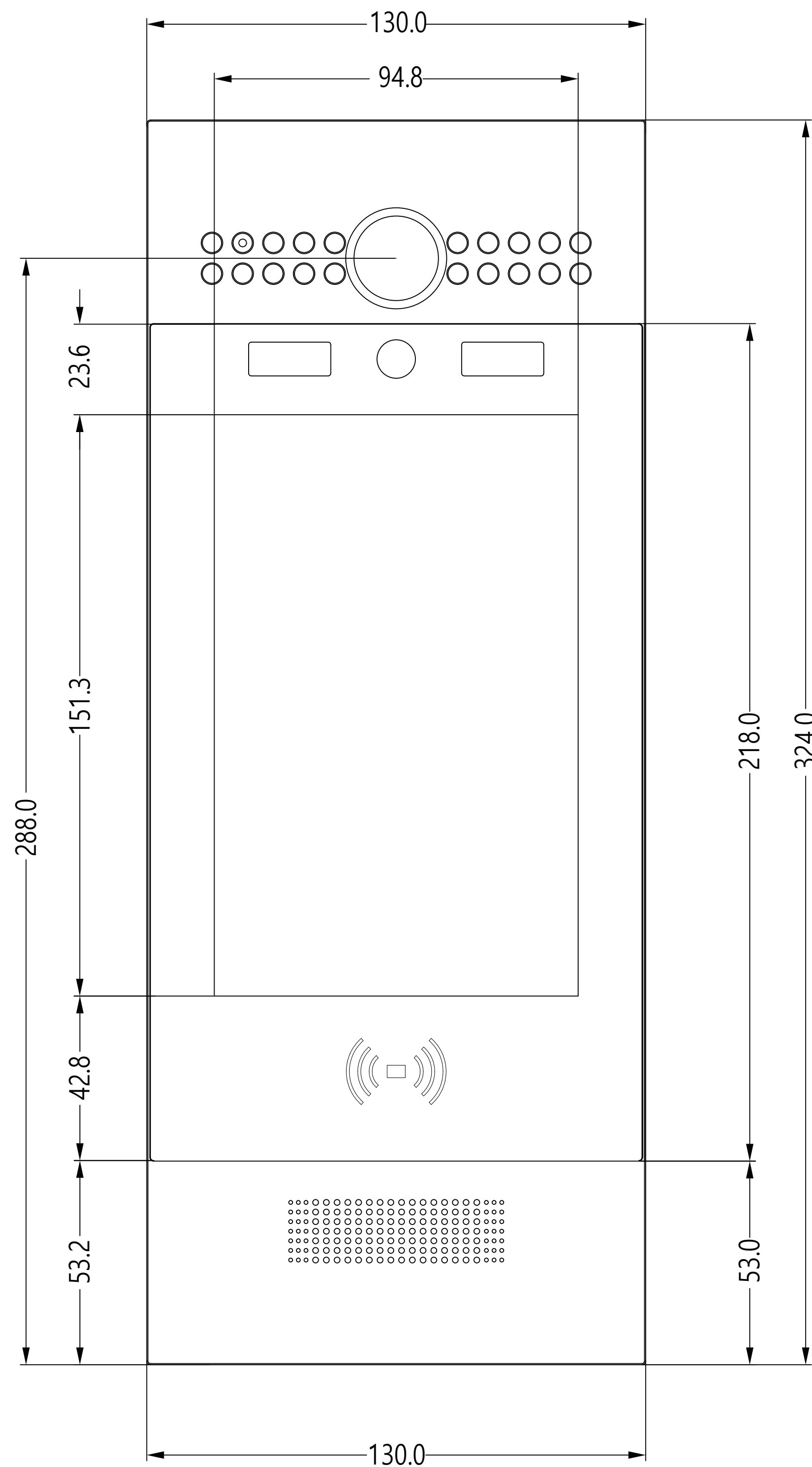
1 FRONT VIEW
