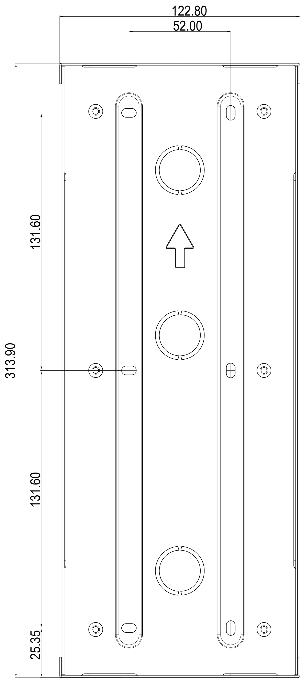
1 FRONT VIEW
