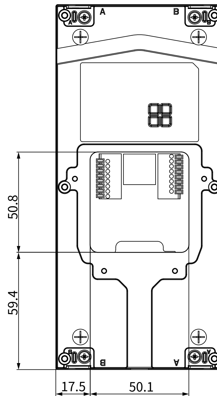
4 BACK VIEW
