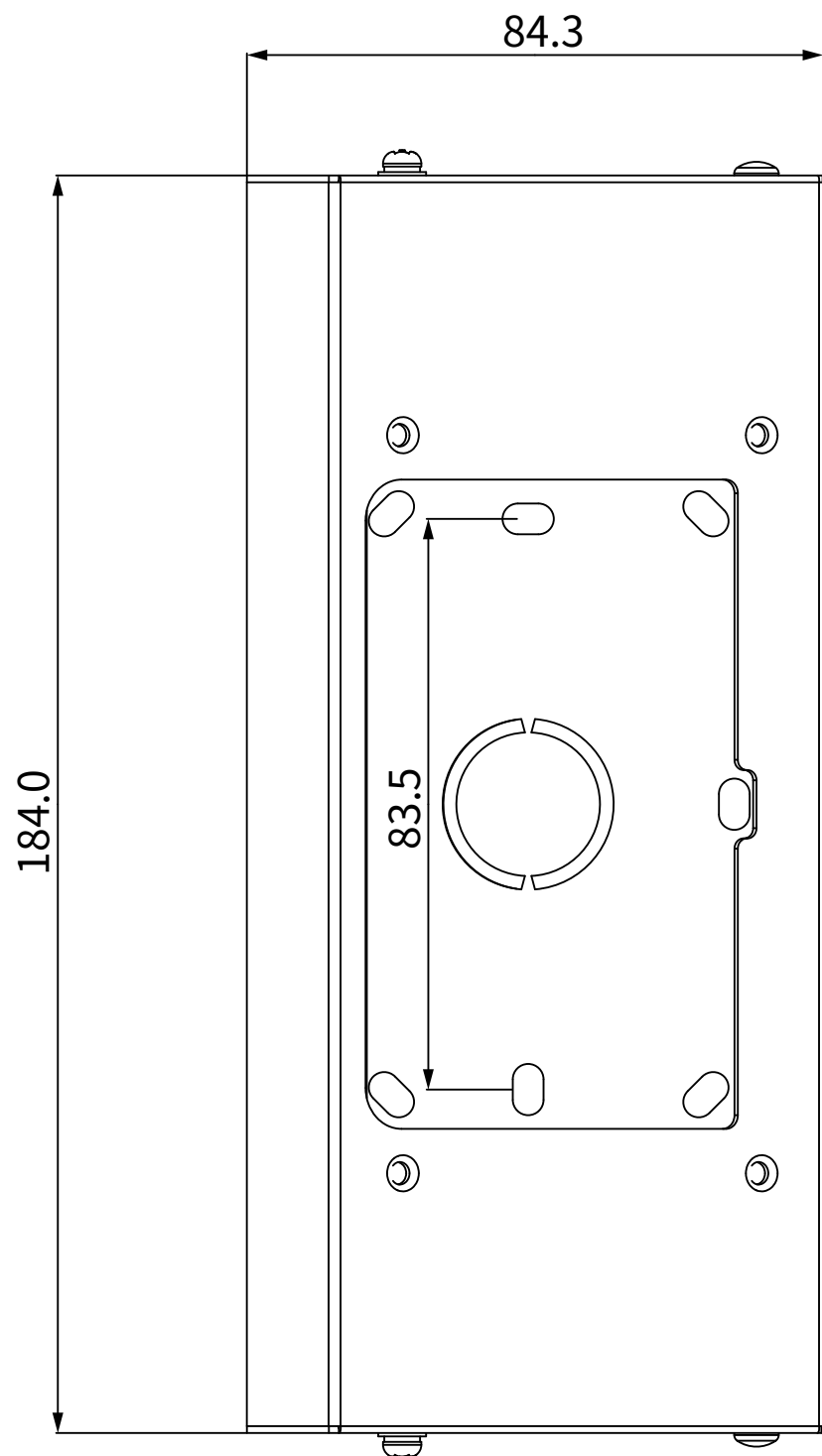
1 FRONT VIEW
