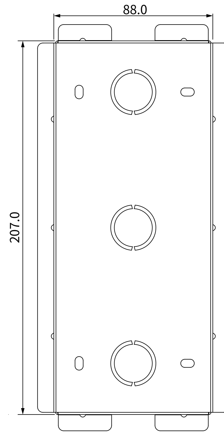
4 BACK VIEW
