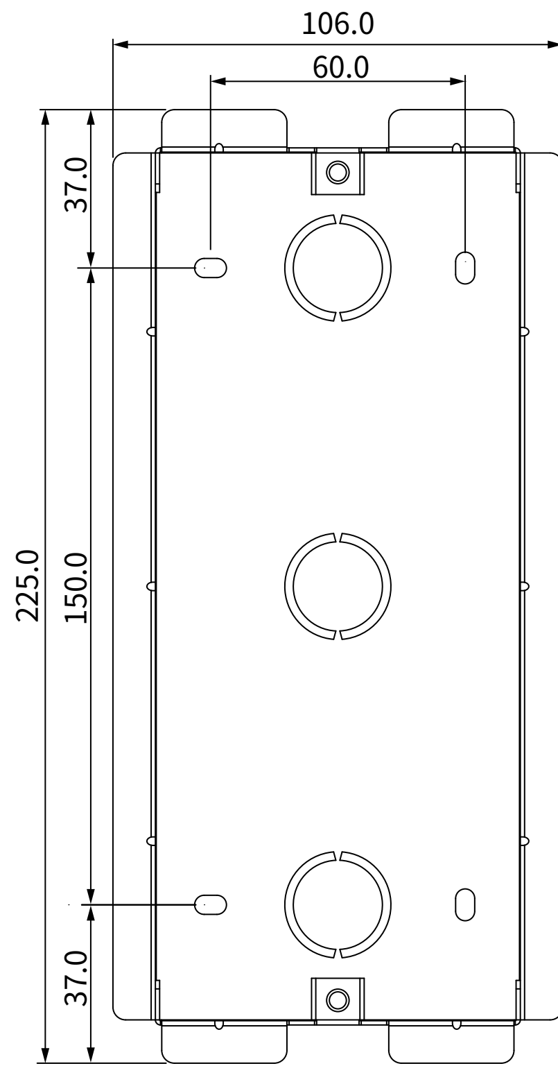
1 FRONT VIEW
