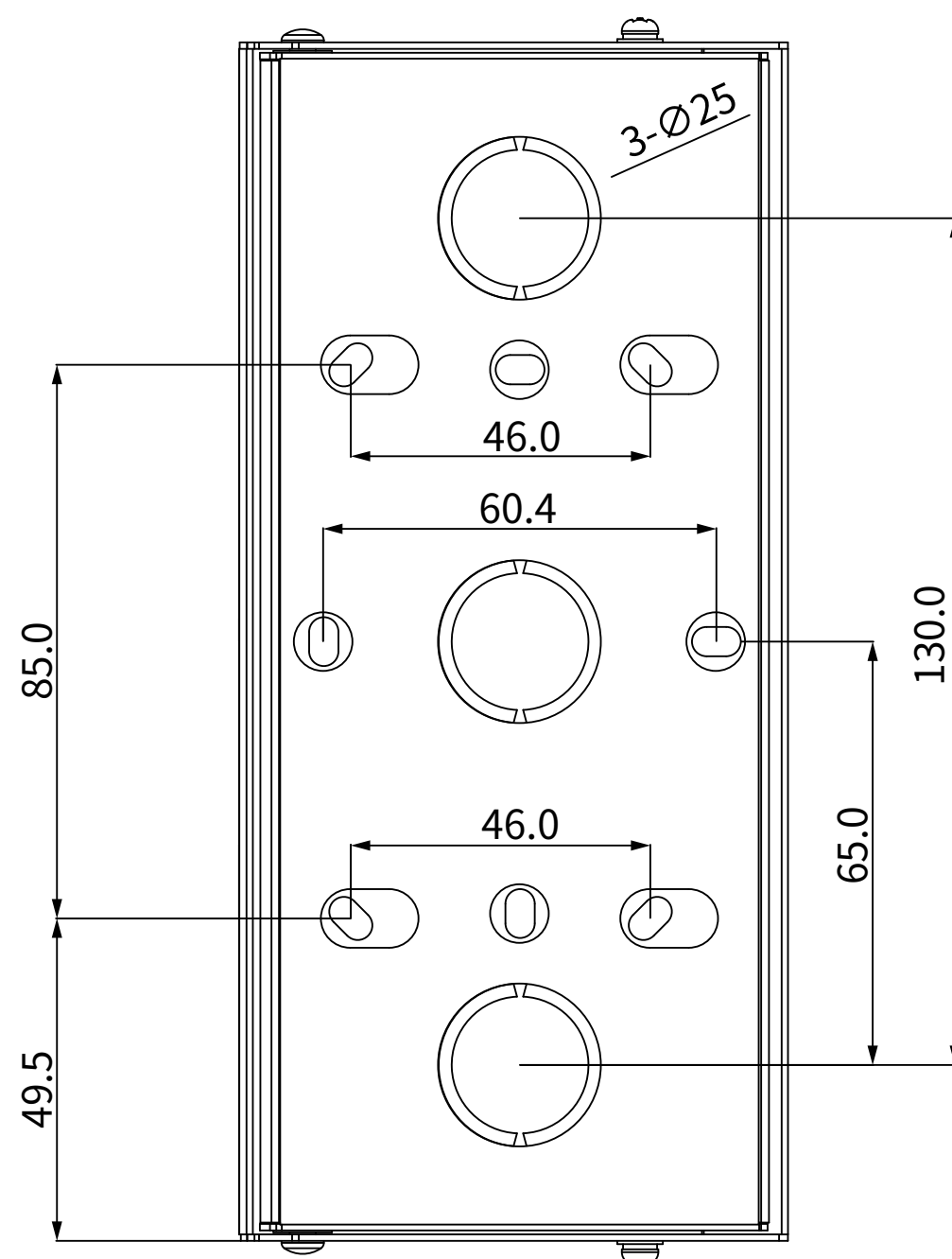
4 BACK VIEW
