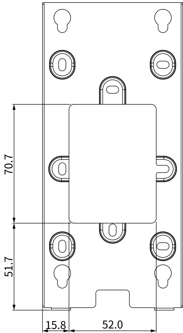
4 BACK VIEW
