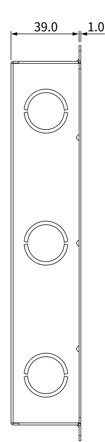
2 RIGHT VIEW
