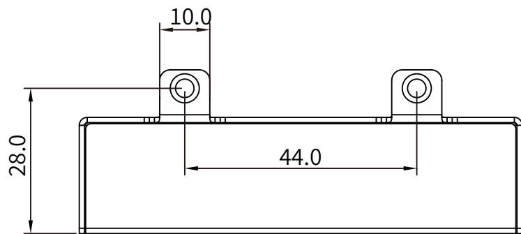
5 TOP VIEW
