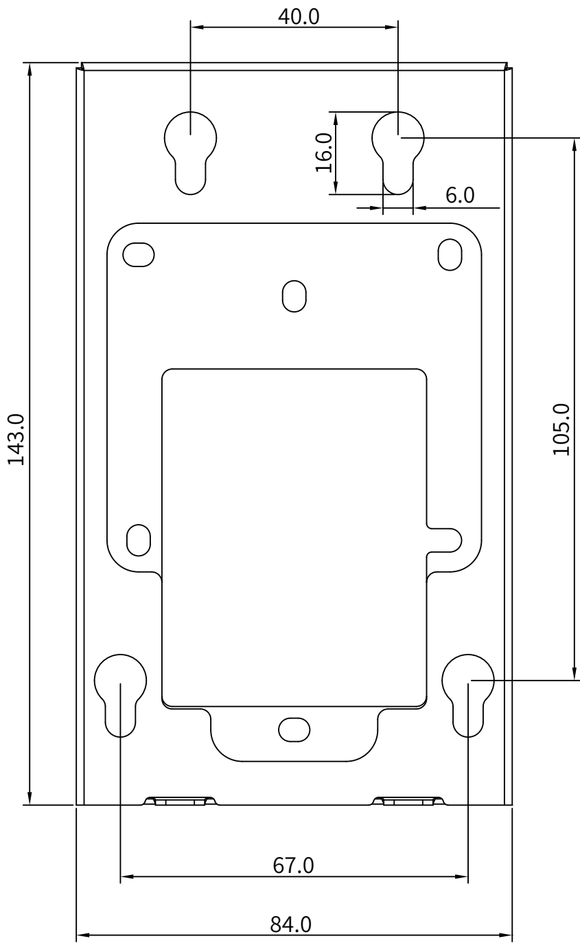
1 FRONT VIEW
