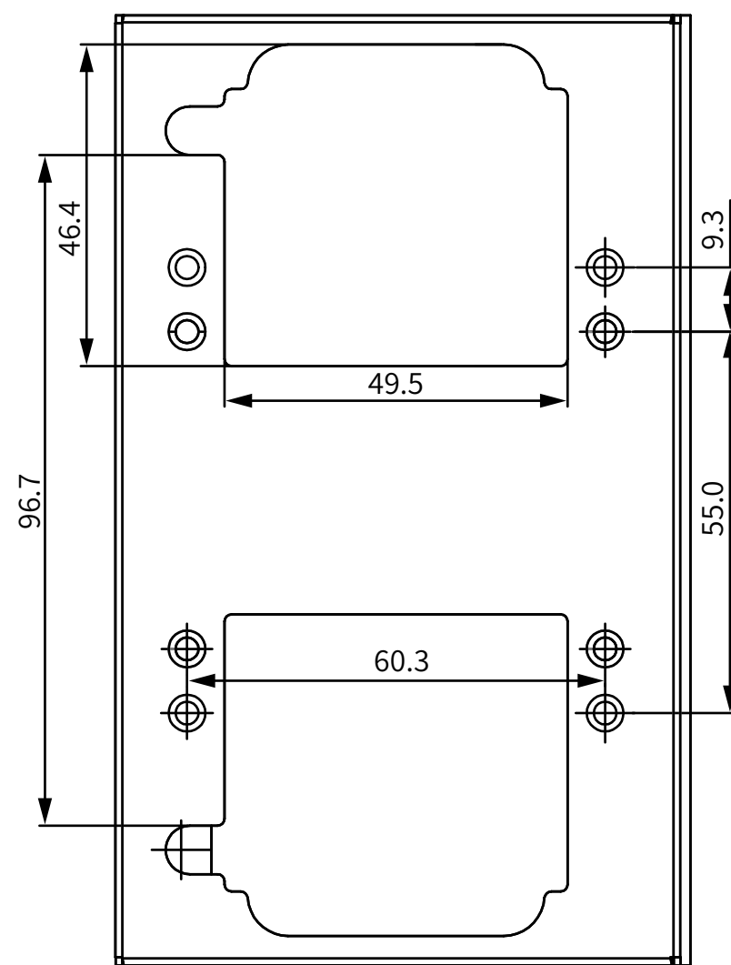
① FRONT VIEW
