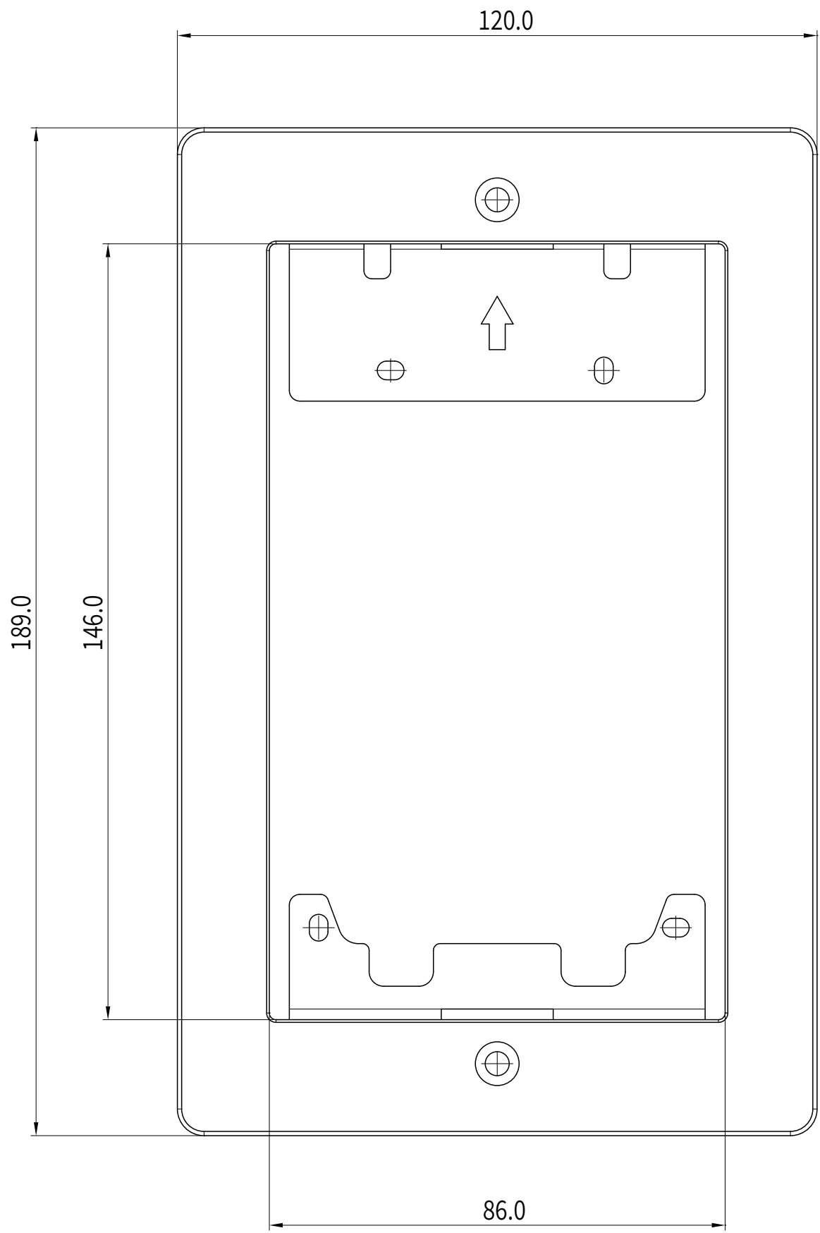
1 FRONT VIEW
