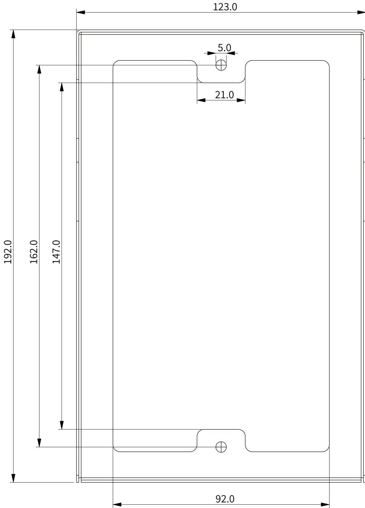
1 FRONT VIEW
