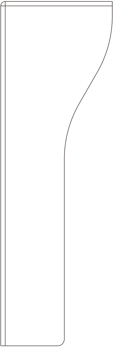
3 LEFT VIEW
