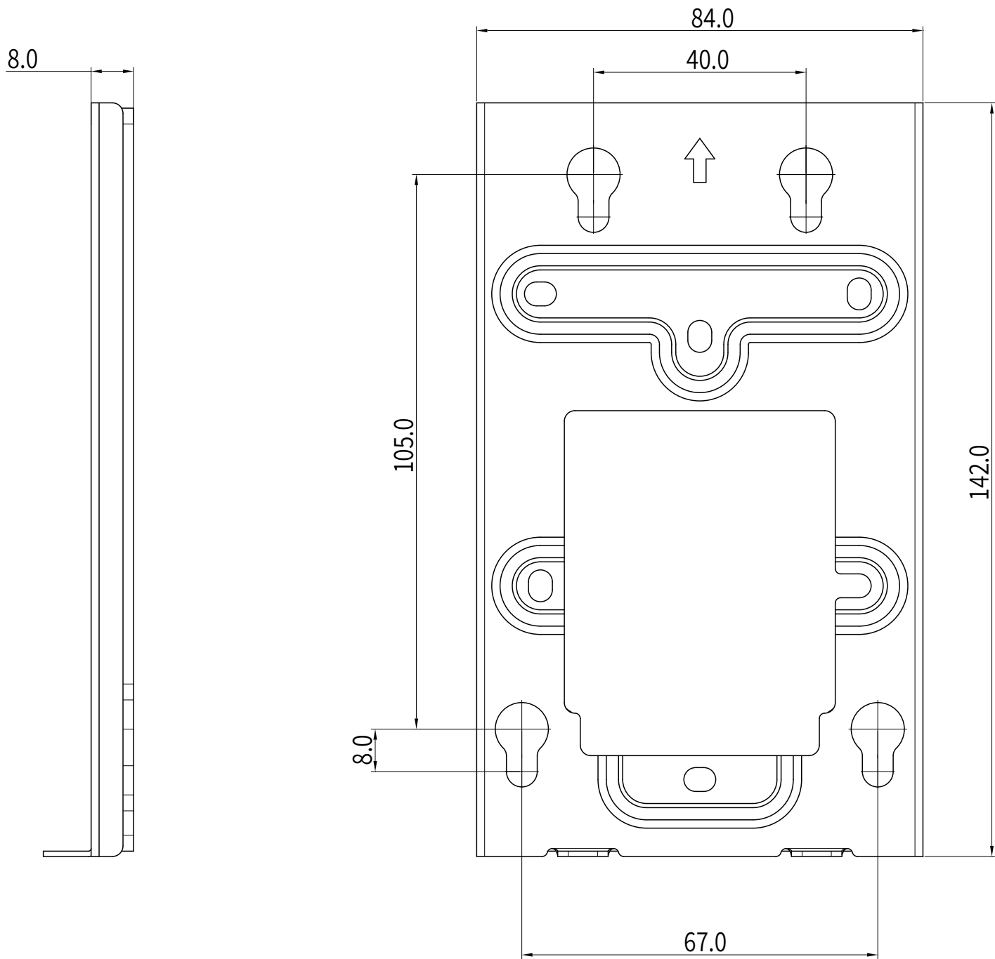
1 FRONT VIEW
