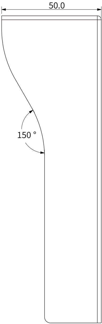
2 RIGHT VIEW
