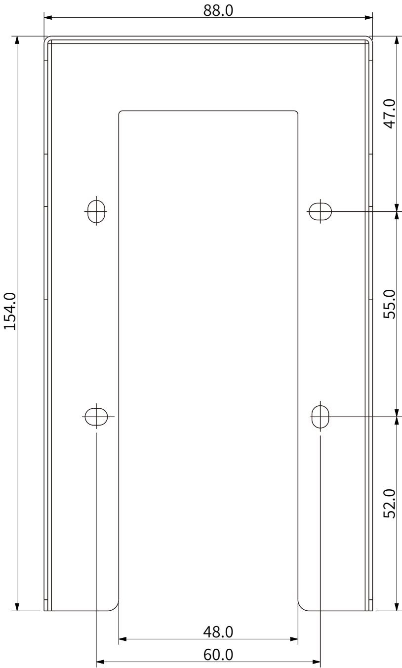
1 FRONT VIEW
