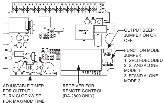
THE MAIN CIRCUIT BOARD OF THE CONTROLLER --- (Figure 2)
